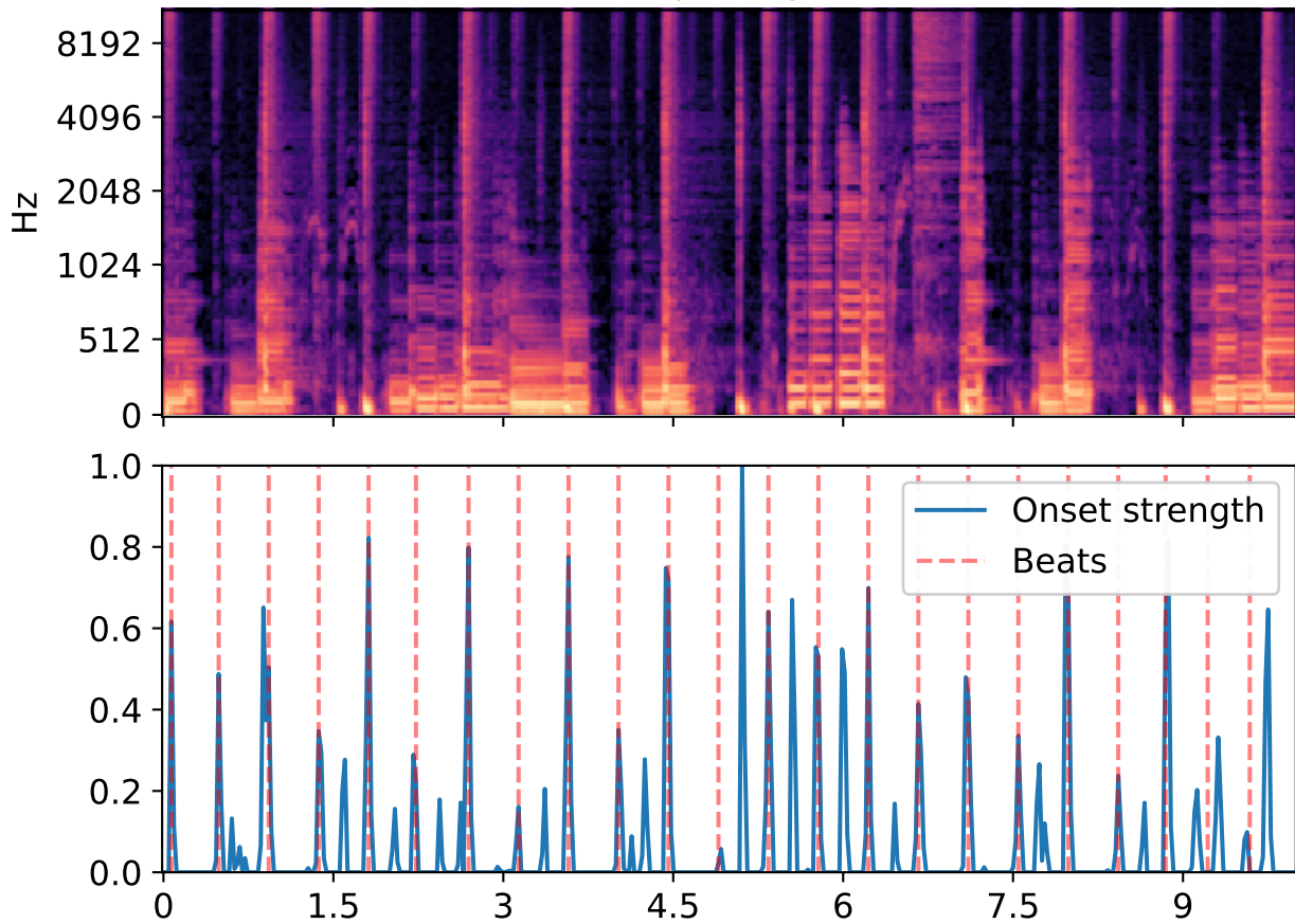
Mel spectrogram
