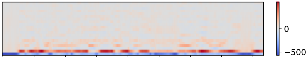
MFCC- \Delta
