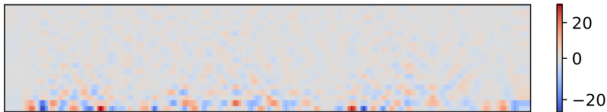
MFCC- \Delta^2
