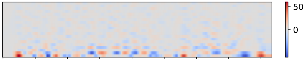
MFCC- \Delta^2
