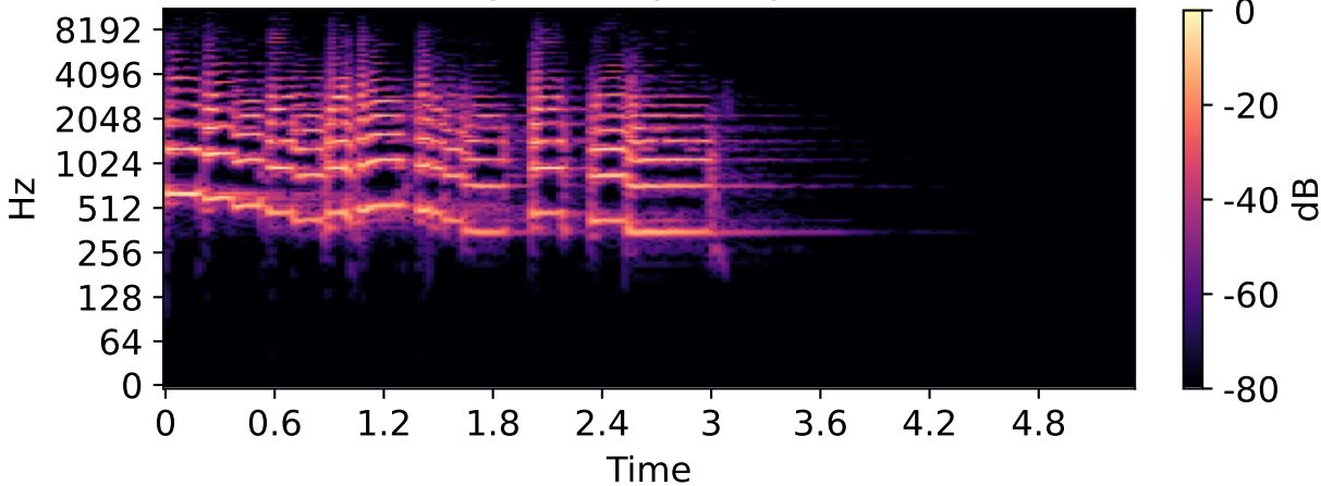
Log-Power spectrogram
