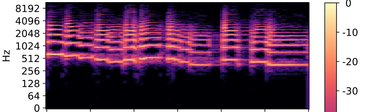
Salience spectrogram
