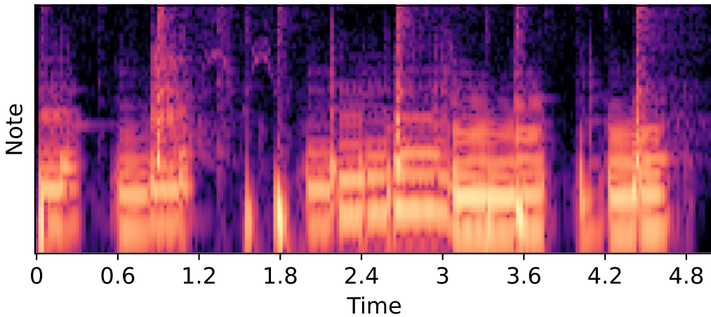
Variable-Q power spectrum
