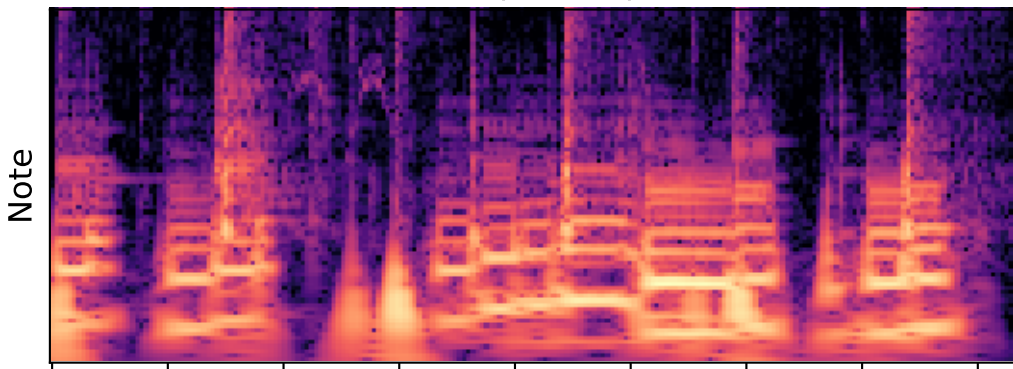
Variable-Q power spectrum
