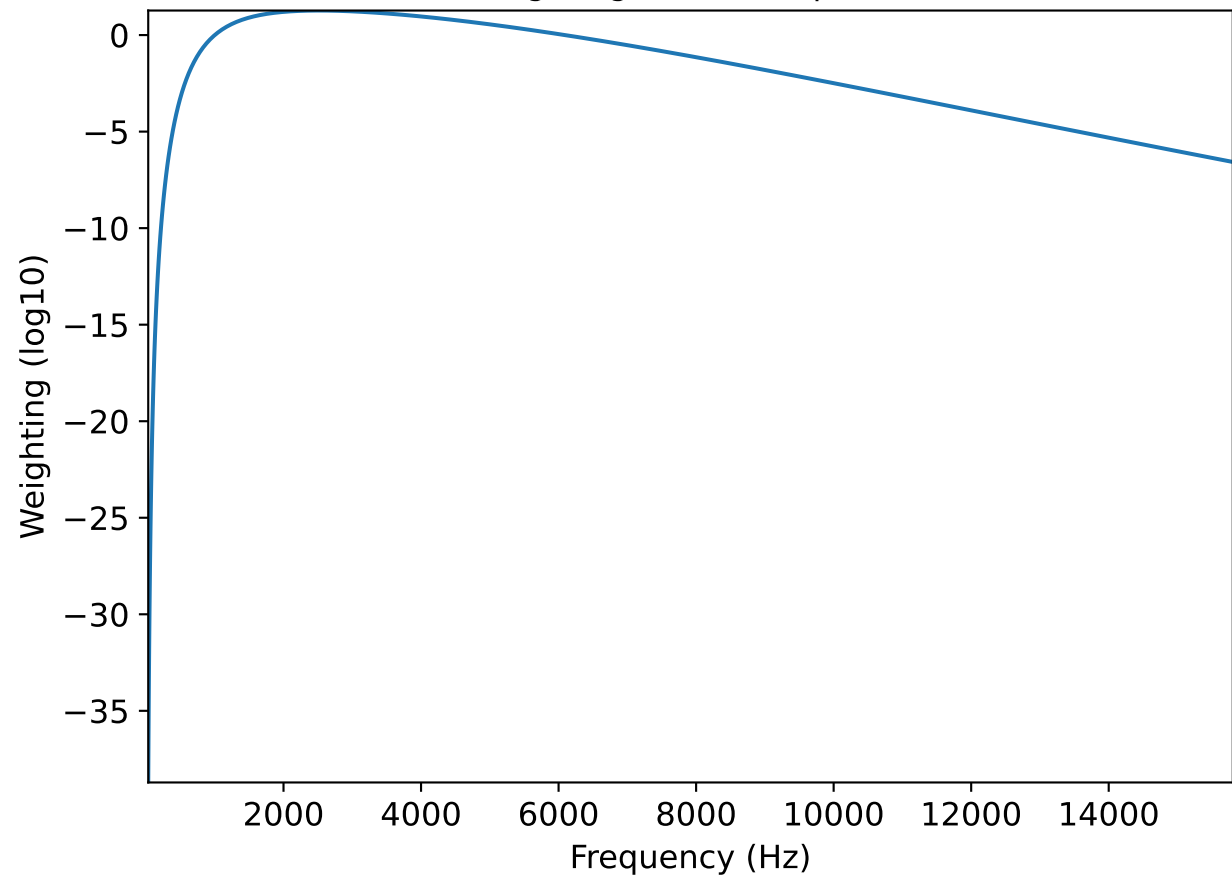
A-Weighting of CQT frequencies
