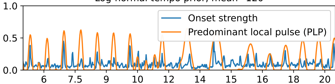
Log-normal tempo prior, mean=120
