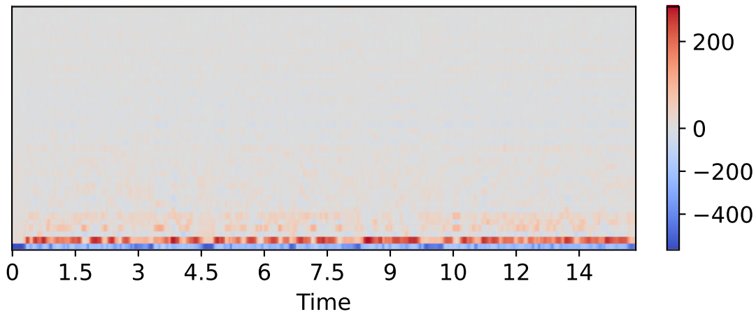
MFCC
