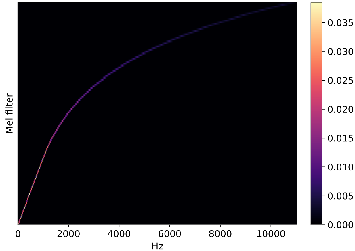
Mel filter bank
