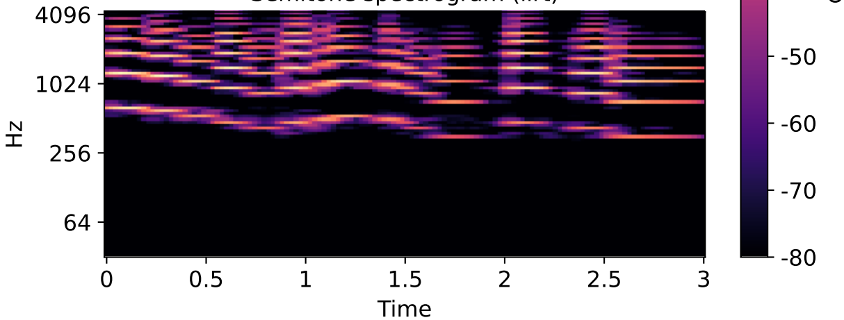
Semitone spectrogram (iirt)
