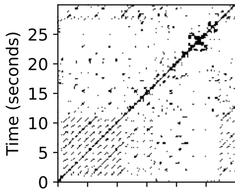
Raw affinity matrix
