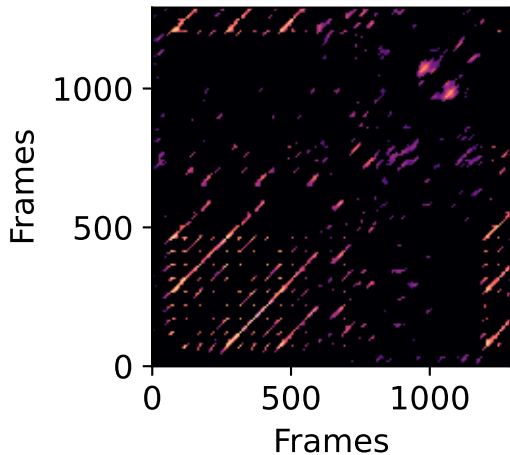
Recurrence matrix
