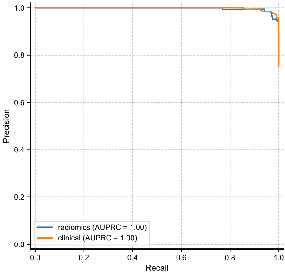
Precision-Recall Curves
