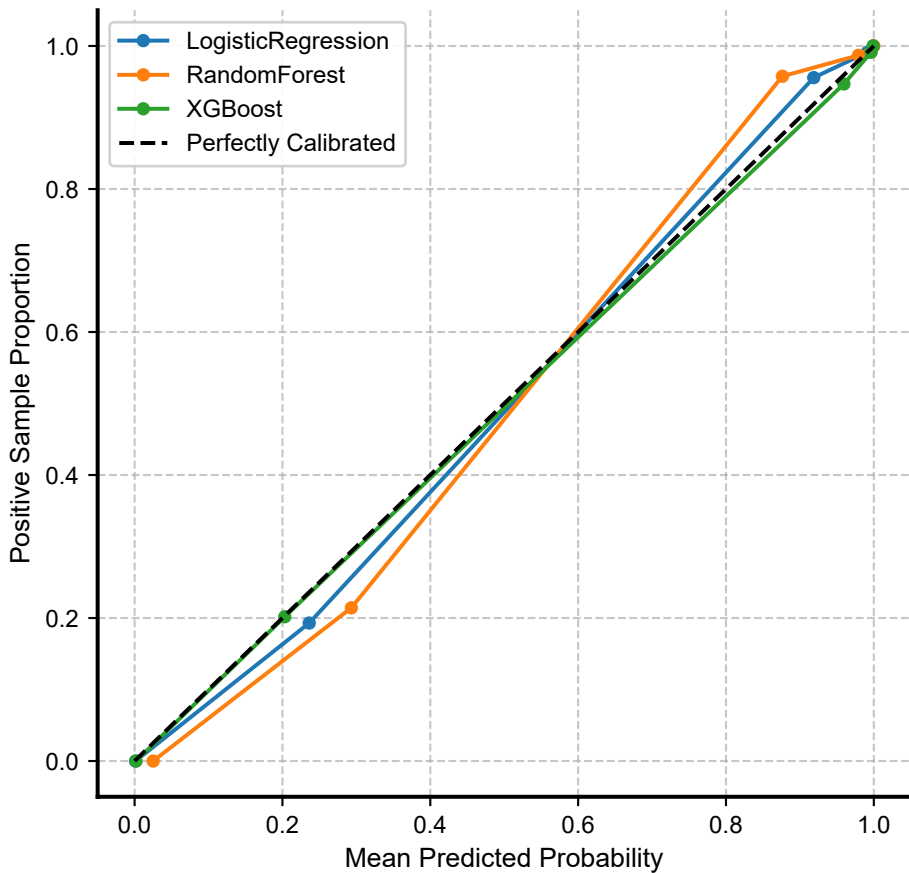
Kfold Calibration
