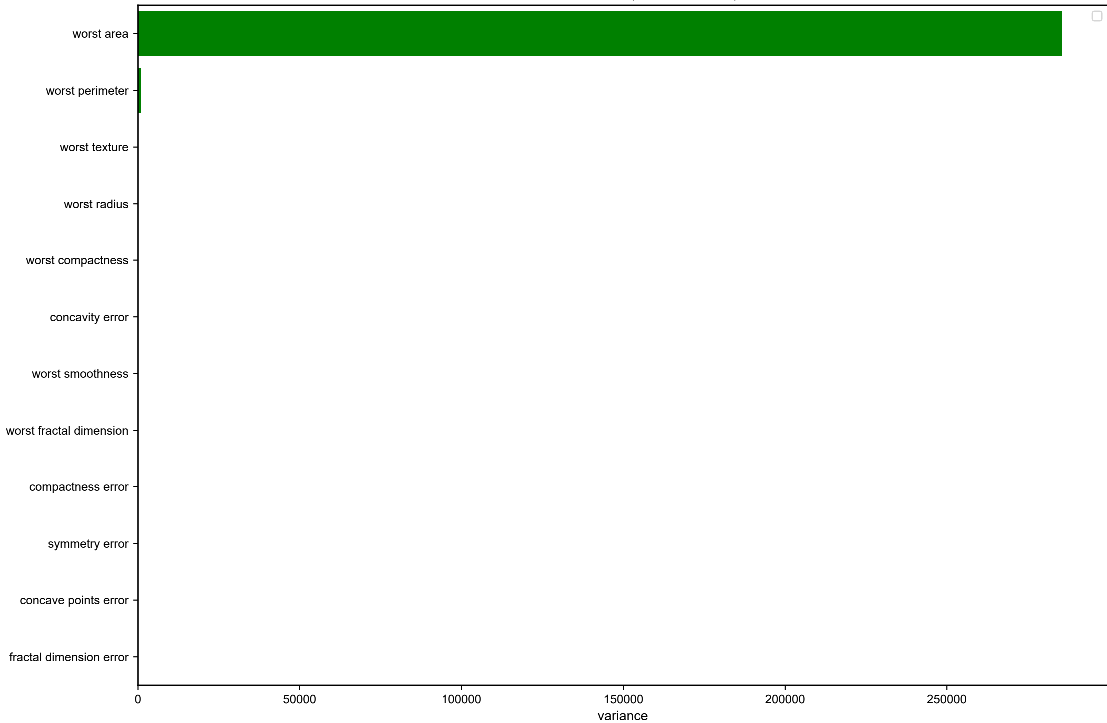
Feature Variances (top 12 selected)
