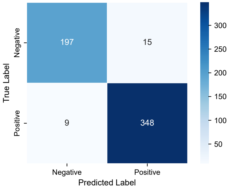
RandomForest - K-Fold CV Confusion Matrix
