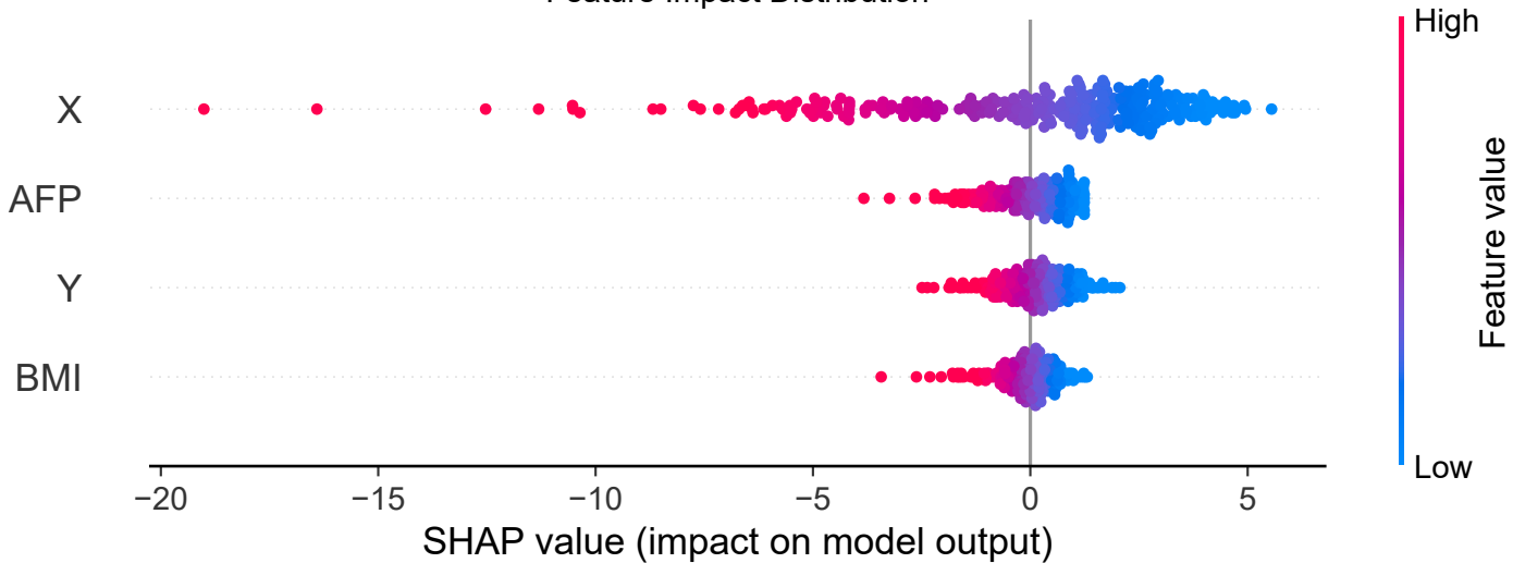
Feature Impact Distribution
