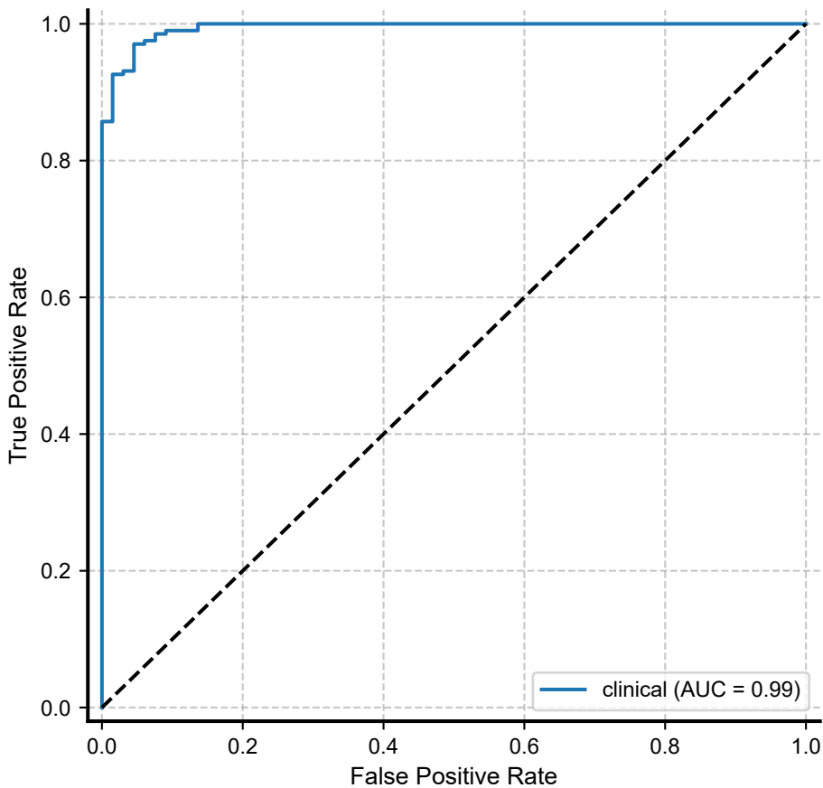
ROC Curves
