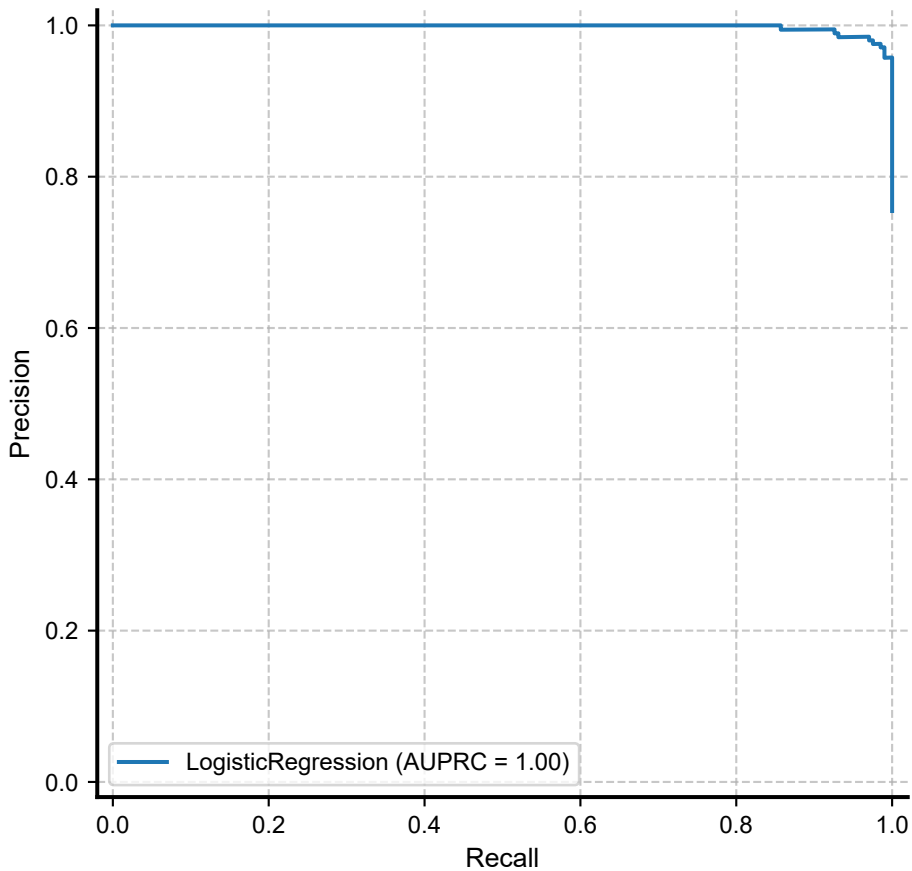
Standard Train PR Curve
