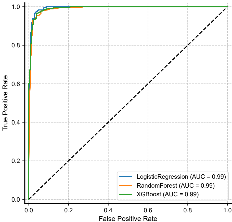
Kfold ROC
