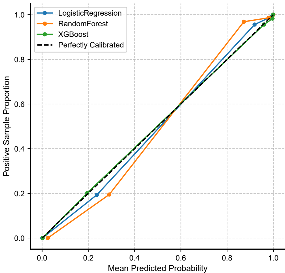
K-Fold Cross-Validation Calibration Curves
