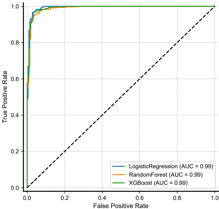
K-Fold Cross-Validation ROC Curves
