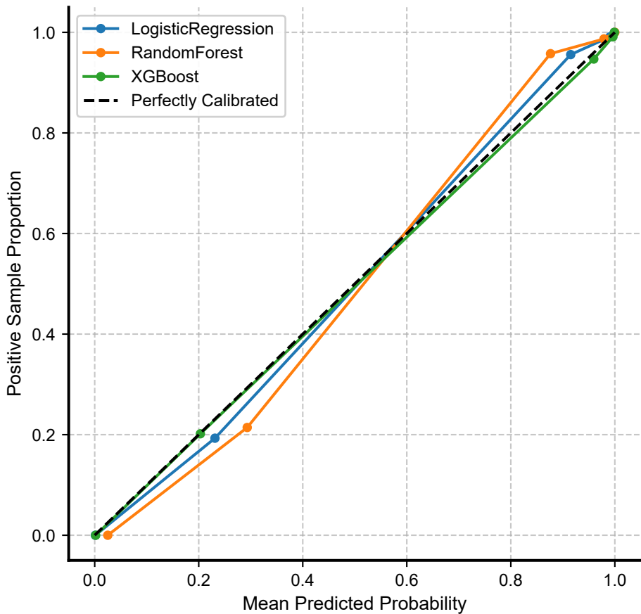
Kfold Calibration
