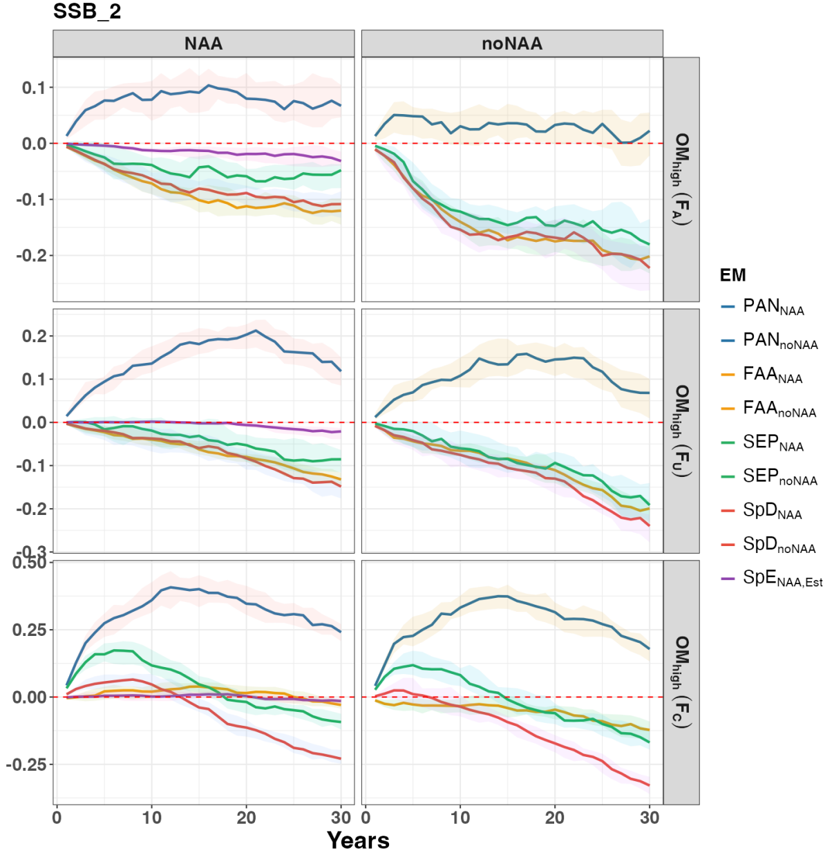
Figure. S10. Relative difference in annual SSB for region 2 between the baseline EM ( SpE_{NAA,Fix} ) and other EMs for each fishing history under the high movement scenario ( OM_{high} ). Each line represents the median trajectory across the 100 realizations, and the shaded area represents the interquartile range (40th–60th percentiles). The performance of EMs with and without NAA random effects is shown separately for better comparison. Three fishing scenarios are included: Adaptive (F A ), Unsustainable (F U ), and Contrasting (F C ).
