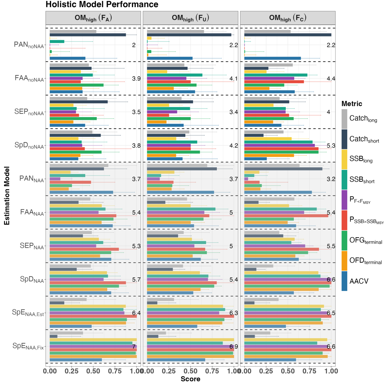
Figure. S14. Overall performance of each EM in region 1 under the high movement scenario ( OM_{high} ), including the following relative performance metrics: 1) long-term catch ( Catch_{long} ); 2) short-term catch ( Catch_{short} ); 3) long-term SSB ( SSB_{long} ); 4) short-term SSB ( SSB_{short} ); 5) probability of F < F_{MSY} ( P_{F < F_{MSY}} ); 6) probability of SSB > SSB_{MSY} ( P_{SSB > SSB_{MSY}} ); 7) overfishing status in the terminal year ( OFG_{terminal} ); 8) overfished status in the terminal year ( OFD_{terminal} ); and 9) average annual catch variation (AACV). Bars represent the median score across the 100 realizations, and error bars represent the interquartile range (25th–75th percentiles). The number displayed in each panel represents the total score (sum of all medians for that EM) for the corresponding EM under that fishing scenario, with higher totals indicating better overall performance. The black dashed line separates the performance of each EM. EMs with a grey background indicate that NAA random effects were included, while EMs with a white background indicate that NAA random effects were not included. Three fishing scenarios are included: Adaptive ( F_A ), Unsustainable ( F_U ), and Contrasting ( F_C ).
