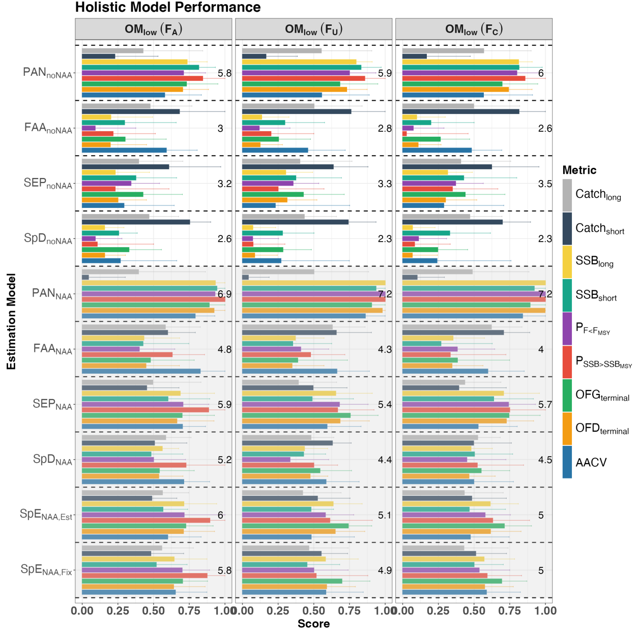
Figure. S35. Overall performance of each EM in region 2 under the low movement scenario ( OM_{low} ), including the following relative performance metrics: 1) long-term catch ( Catch_{long} ); 2) short-term catch ( Catch_{short} ); 3) long-term SSB ( SSB_{long} ); 4) short-term SSB ( SSB_{short} ); 5) probability of F < F_{MSY} ( P_{F < F_{MSY}} ); 6) probability of SSB > SSB_{MSY} ( P_{SSB > SSB_{MSY}} ); 7) overfishing status in the terminal year ( OFG_{terminal} ); 8) overfished status in the terminal year ( OFD_{terminal} ); and 9) average annual catch variation (AACV). Bars represent the median score across the 100 realizations, and error bars represent the interquartile range (25th–75th percentiles). The number displayed in each panel represents the total score (sum of all medians for that EM) for the corresponding EM under that fishing scenario, with higher totals indicating better overall performance. The black dashed line separates the performance of each EM. EMs with a grey background indicate that NAA random effects were included, while EMs with a white background indicate that NAA random effects were not included. Three fishing scenarios are included: Adaptive ( F_A ), Unsustainable ( F_U ), and Contrasting ( F_C ).
