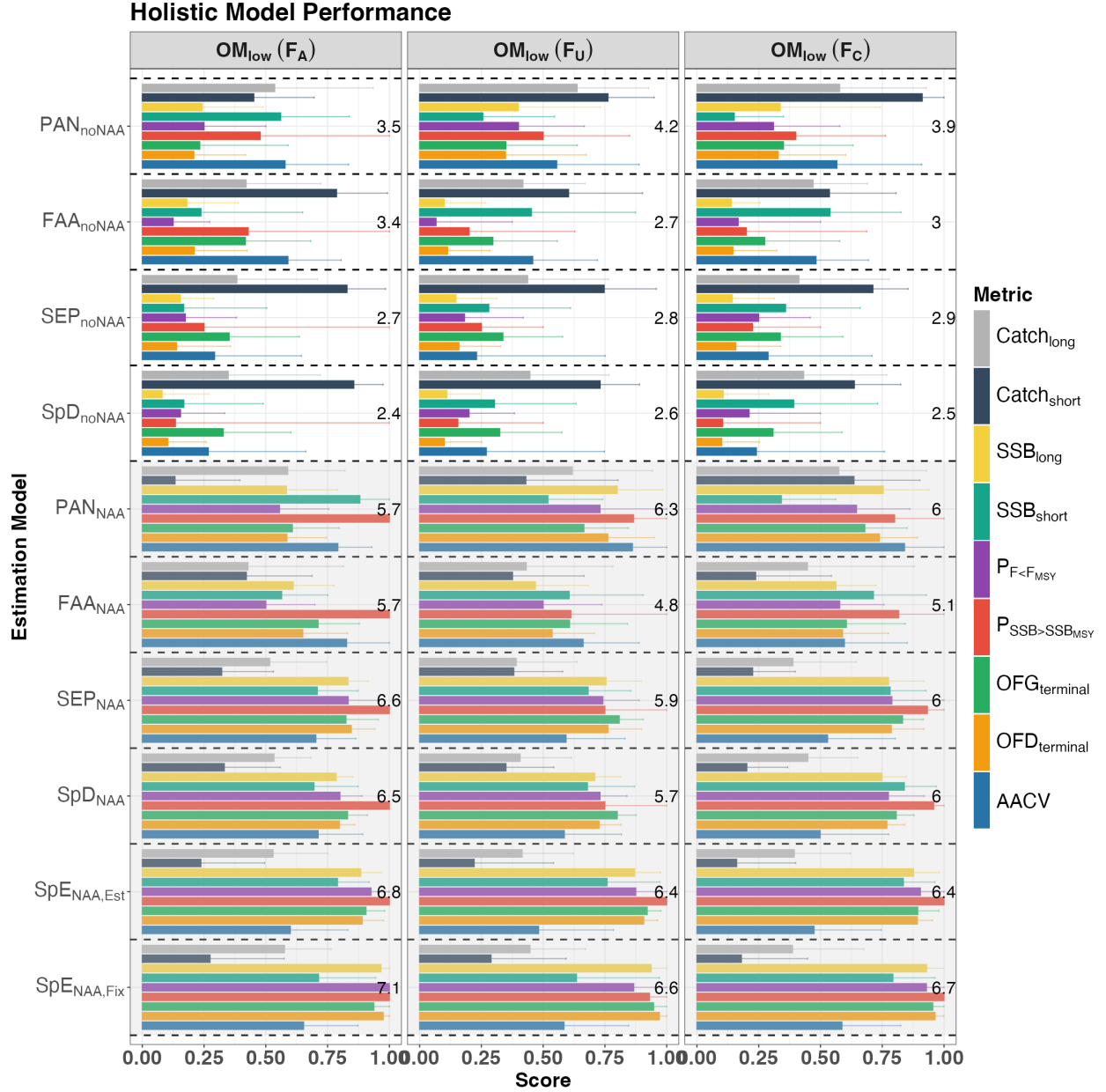
Figure. S33. Overall performance of each EM at the global scale under the low movement scenario (OM low ), including the following relative performance metrics: 1) long-term catch (Catch long ); 2) short-term catch (Catch short ); 3) long-term SSB (SSB long ); 4) short-term SSB (SSB short ); 5) probability of F < F_{MSY} ( P_{F < F_{MSY}} ); 6) probability of SSB > SSB_{MSY} ( P_{SSB > SSB_{MSY}} ); 7) overfishing status in the terminal year (OFG terminal ); 8) overfished status in the terminal year (OFD terminal ); and 9) average annual catch variation (AACV). Bars represent the median score across the 100 realizations, and error bars represent the interquartile range (25th–75th percentiles). The number displayed in each panel represents the total score (sum of all medians for that EM) for the corresponding EM under that fishing scenario, with higher totals indicating better overall performance. The black dashed line separates the performance of each EM. EMs with a grey background indicate that NAA random effects were included, while EMs with a white background indicate that NAA random effects were not included. Three fishing scenarios are included: Adaptive (F A ), Unsustainable (F U ), and Contrasting (F C ).
