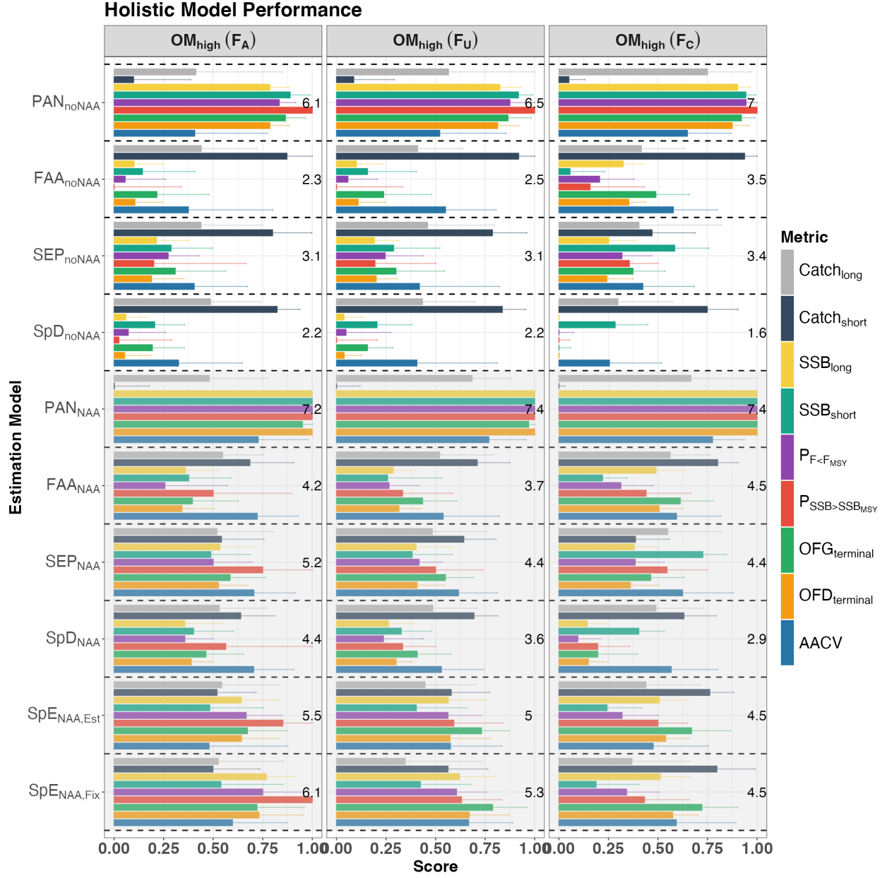
Figure. S15. Overall performance of each EM in region 2 under the high movement scenario ( OM_{high} ), including the following relative performance metrics: 1) long-term catch ( Catch_{long} ); 2) short-term catch ( Catch_{short} ); 3) long-term SSB ( SSB_{long} ); 4) short-term SSB ( SSB_{short} ); 5) probability of F < F_{MSY} ( P_{F < F_{MSY}} ); 6) probability of SSB > SSB_{MSY} ( P_{SSB > SSB_{MSY}} ); 7) overfishing status in the terminal year ( OFG_{terminal} ); 8) overfished status in the terminal year ( OFD_{terminal} ); and 9) average annual catch variation (AACV). Bars represent the median score across the 100 realizations, and error bars represent the interquartile range (25th–75th percentiles). The number displayed in each panel represents the total score (sum of all medians for that EM) for the corresponding EM under that fishing scenario, with higher totals indicating better overall performance. The black dashed line separates the performance of each EM. EMs with a grey background indicate that NAA random effects were included, while EMs with a white background indicate that NAA random effects were not included. Three fishing scenarios are included: Adaptive ( F_A ), Unsustainable ( F_U ), and Contrasting ( F_C ).
