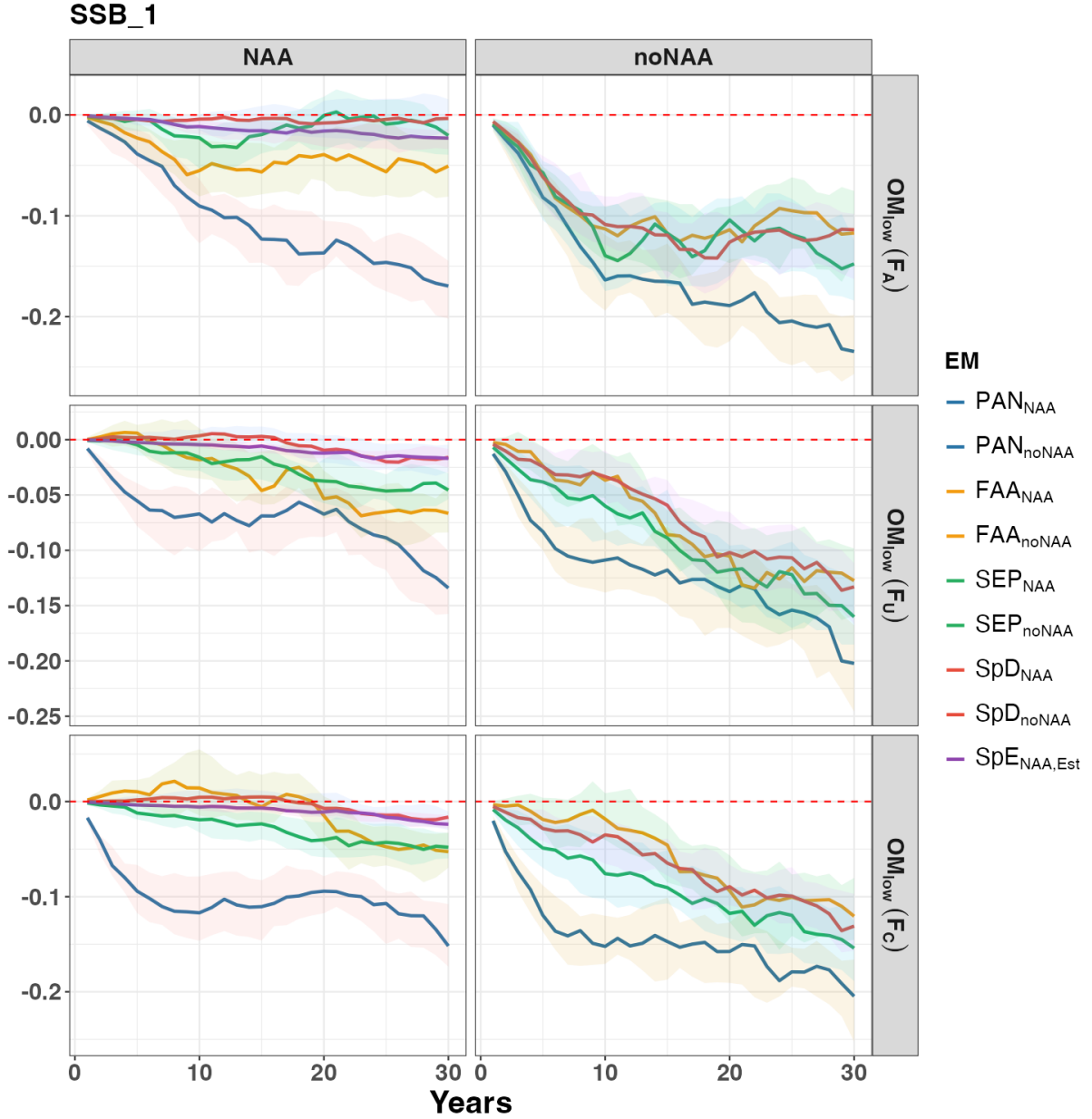
Figure. S24. Relative difference in annual SSB for region 1 between the baseline EM ( SpE_{NAA,Fix} ) and other EMs for each fishing history under the low movement scenario ( OM_{low} ). Each line represents the median trajectory across the 100 realizations, and the shaded area represents the interquartile range (40th–60th percentiles). The performance of EMs with and without NAA random effects is shown separately for better comparison. Three fishing scenarios are included: Adaptive ( F_A ), Unsustainable ( F_U ), and Contrasting ( F_C ).
