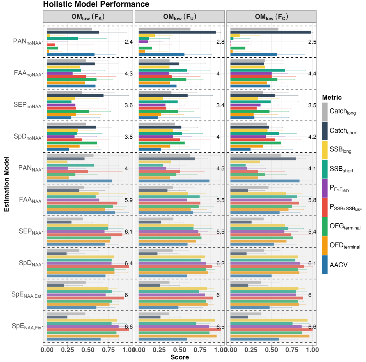
Figure. S34. Overall performance of each EM in region 1 under the low movement scenario (OM low ), including the following relative performance metrics: 1) long-term catch (Catch long ); 2) short-term catch (Catch short ); 3) long-term SSB (SSB long ); 4) short-term SSB (SSB short ); 5) probability of F < F_{MSY} ( P_{F < F_{MSY}} ); 6) probability of SSB > SSB_{MSY} ( P_{SSB > SSB_{MSY}} ); 7) overfishing status in the terminal year (OFG terminal ); 8) overfished status in the terminal year (OFD terminal ); and 9) average annual catch variation (AACV). Bars represent the median score across the 100 realizations, and error bars represent the interquartile range (25th–75th percentiles). The number displayed in each panel represents the total score (sum of all medians for that EM) for the corresponding EM under that fishing scenario, with higher totals indicating better overall performance. The black dashed line separates the performance of each EM. EMs with a grey background indicate that NAA random effects were included, while EMs with a white background indicate that NAA random effects were not included. Three fishing scenarios are included: Adaptive (F A ), Unsustainable (F U ), and Contrasting (F C ).
