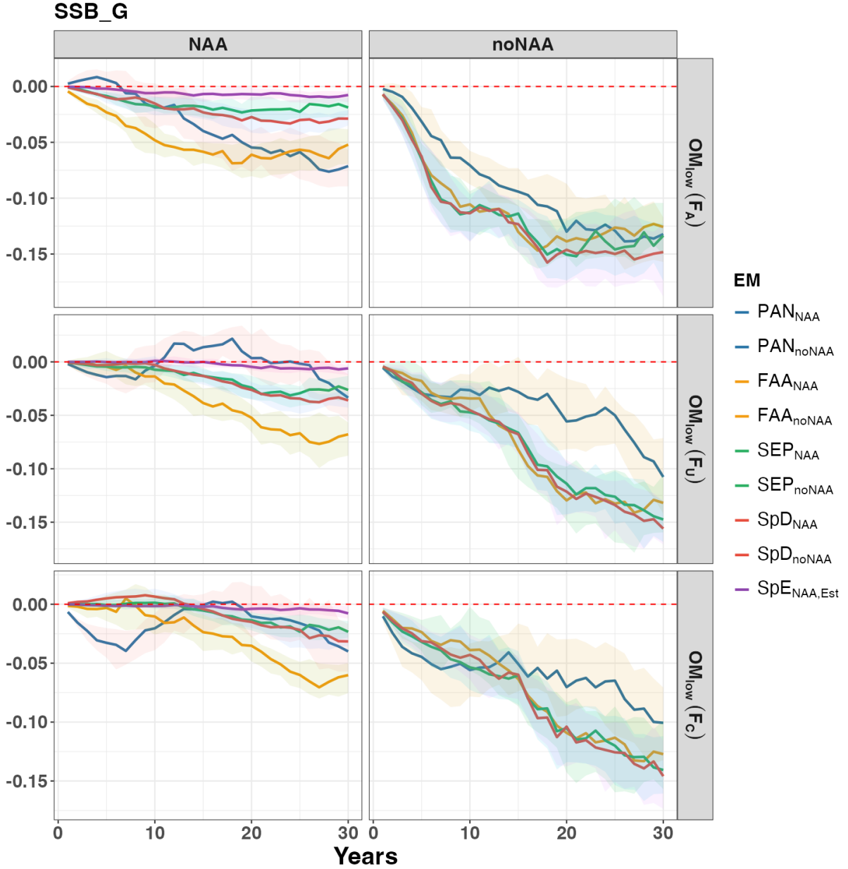
Figure. S23. Relative difference in annual total SSB between the baseline EM ( SpE_{NAA,Fix} ) and other EMs for each fishing history under the low movement scenario ( OM_{low} ). Each line represents the median trajectory across the 100 realizations, and the shaded area represents the interquartile range (40th–60th percentiles). The performance of EMs with and without NAA random effects is shown separately for better comparison. Three fishing scenarios are included: Adaptive ( F_A ), Unsustainable ( F_U ), and Contrasting ( F_C ).
