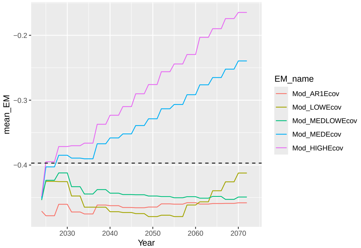
Figure 1: Estimated ecological covariates in for the different temperature projection choices in the EM compared to the “true” value in the OM.
