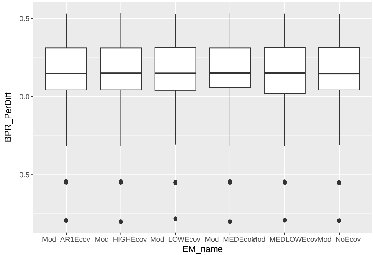
Figure 5: Percent difference of the calculated FXSPR reference point in each EM compared to the OM.
