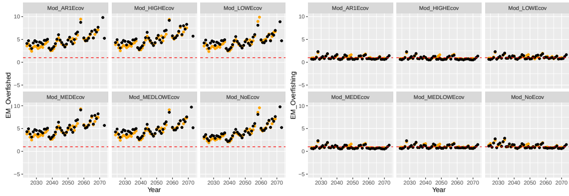
Figure 4: Overfished (left) and overfishing (right) status over the projected time series for each EM. Overfished and overfishing thresholds are shown in the horizontal red line
