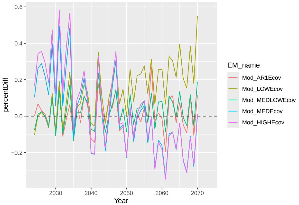
Figure 2: Percent difference of the calculated recruitment per assessment year in each EM compared to the OM.
