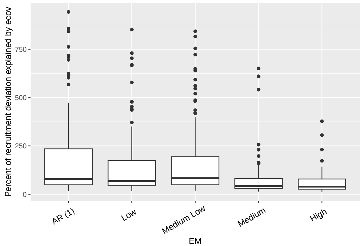
Figure 3: Percent of recruitment deviation EXPLAINED BY THE ECOV IN EACH MODEL. MAKE SURE YOU CHANGE YOUR RESULTS PARAGRAPHS TO SAY THIS. ALSO FIX THIS BASED ON CHENG EMAIL
