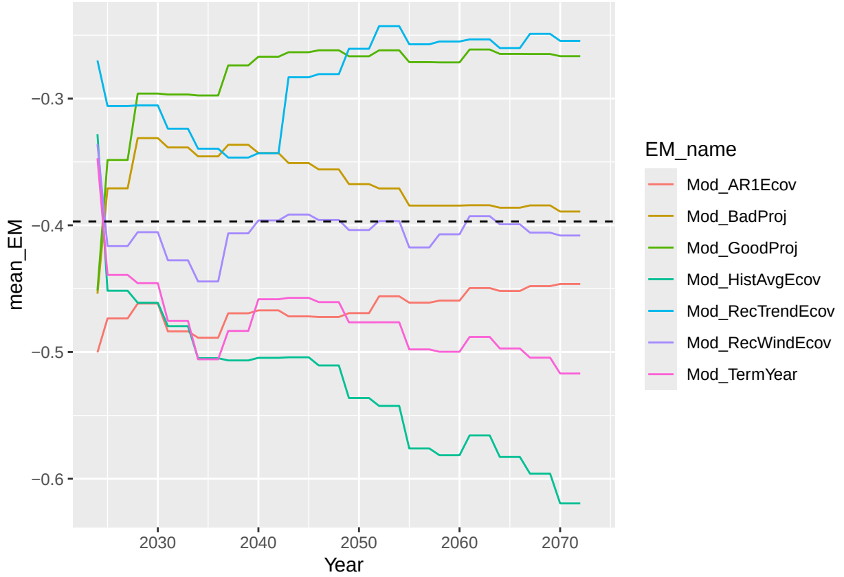
Figure 1: Estimated ecological covariates in for the different temperature projection choices in the EM compared to the “true” value in the OM.
