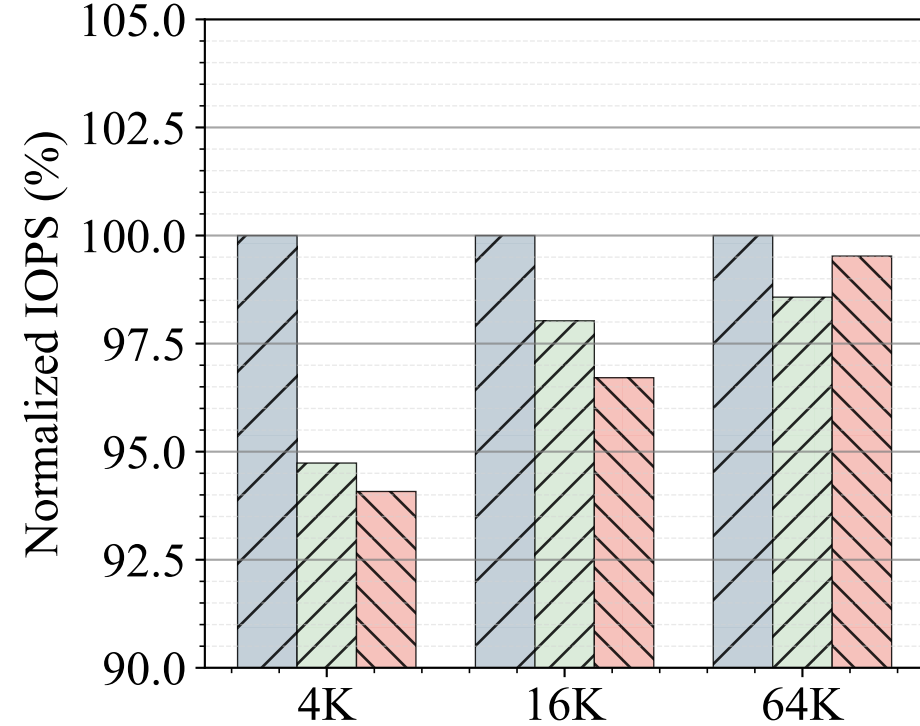
(b) Random Write IOPS
