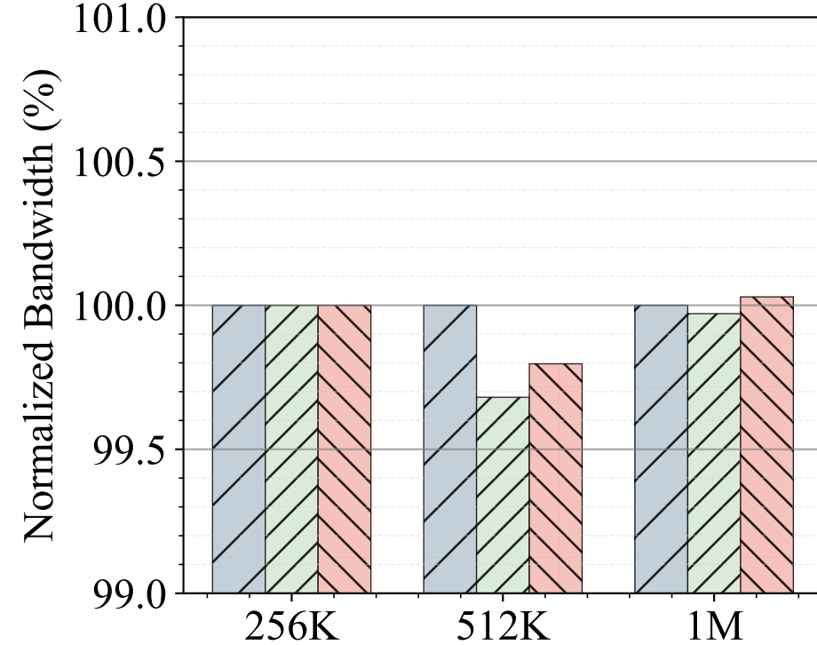
(c) Sequential Read Bandwidth
