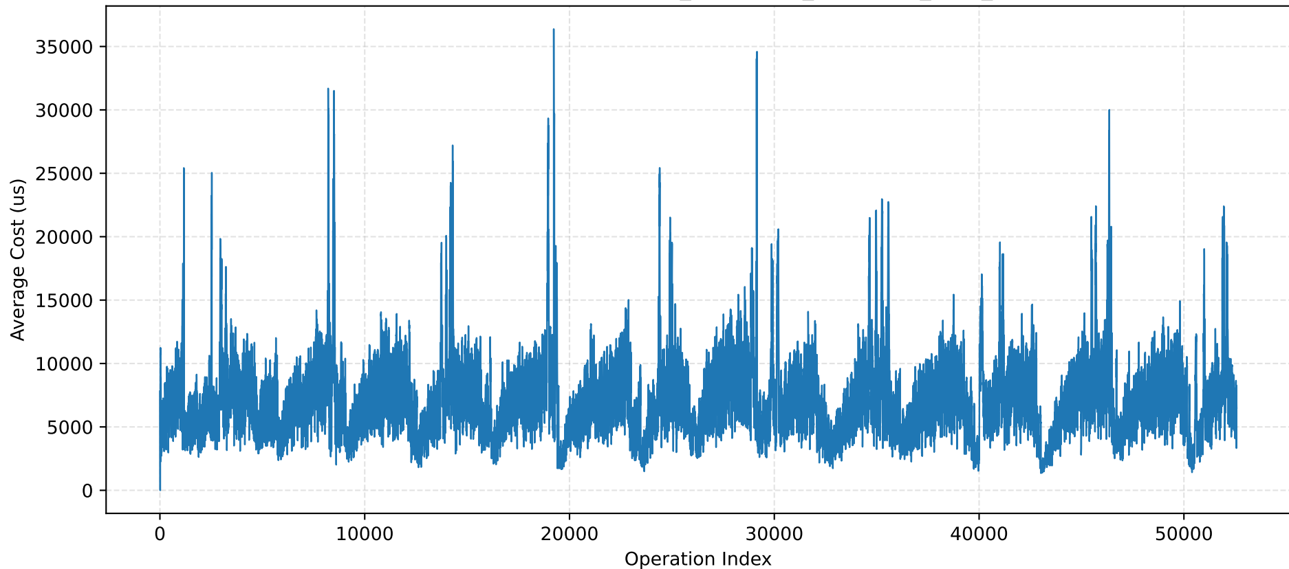
Average Latency Trend of t4_log and t5_log - btrfs_sync_file
