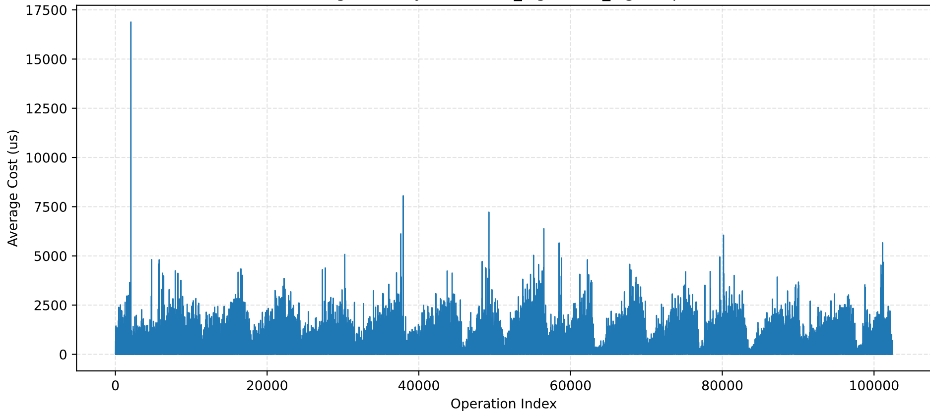
Average Latency Trend of t4_log and t5_log - req4096
