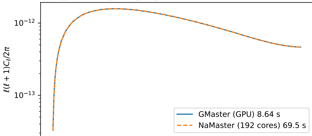
y_unlensed_L2p8_m9_lc0.fits, TT, nside 4096, nlb 50
