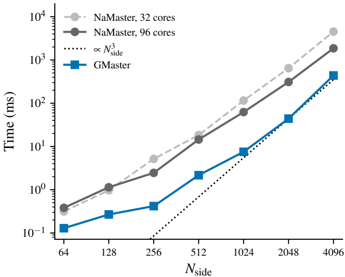
spin 0
