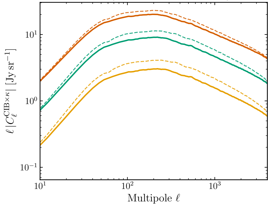
CIB- \kappa (cf. Yang26 Fig. 10 right)
