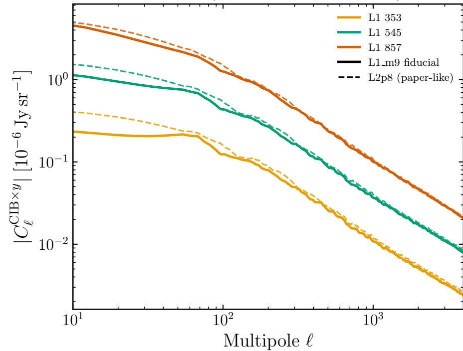
CIB-tSZ (cf. Yang26 Fig. 10 left)
