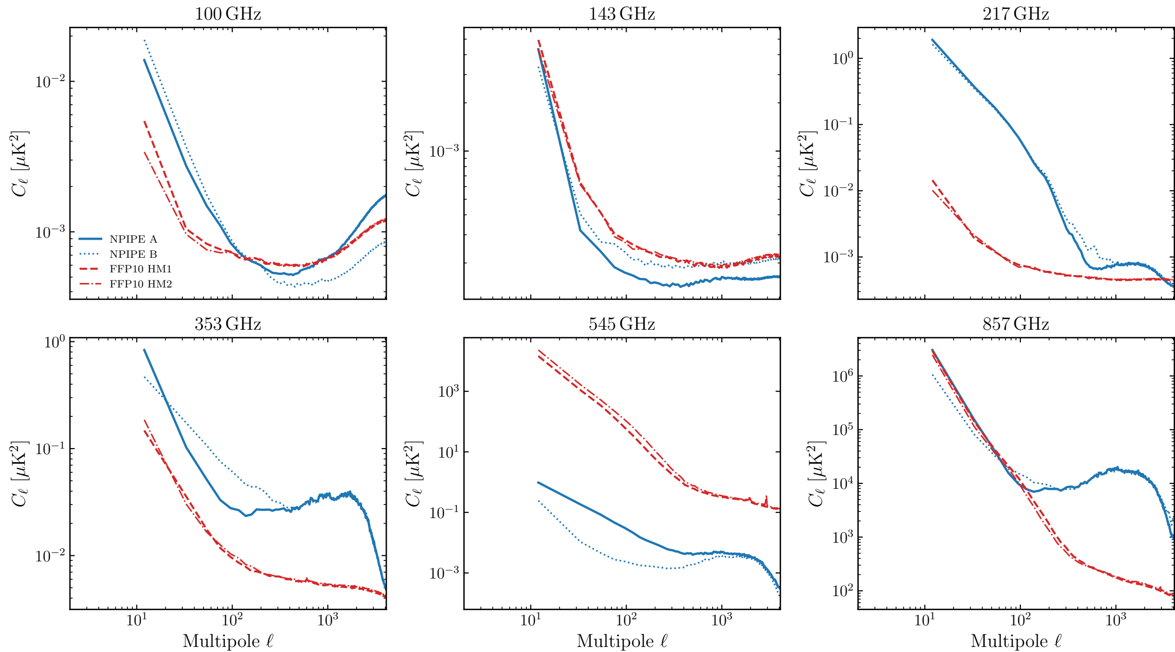
NPIPE A/B vs FFP10 HM1/HM2 noise auto-spectra
