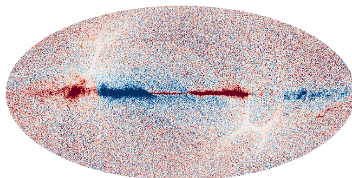
FFP10 HM1 545 GHz
