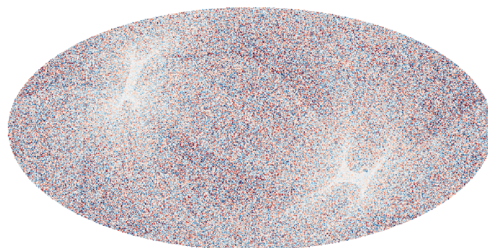
FFP10 HM1 217 GHz
