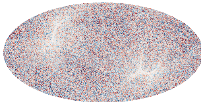
FFP10 HM1 143 GHz
