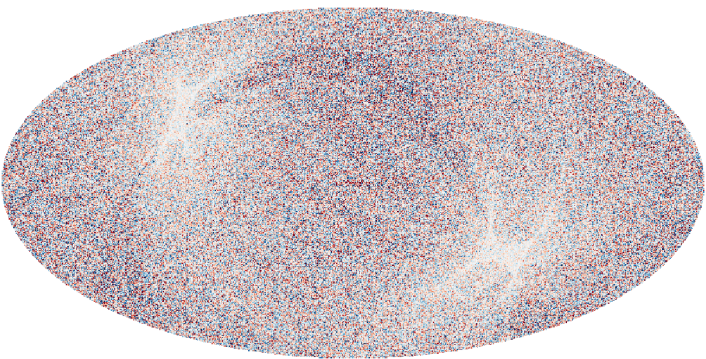
Noise residual, shared colour scale per frequency (mc 00200 vs mc 00000)
