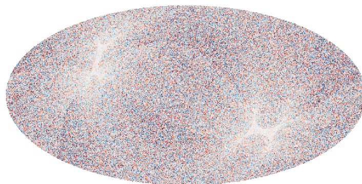
FFP10 HM1 353 GHz
