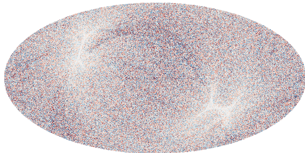
143 GHz NPIPE A mc_00200
