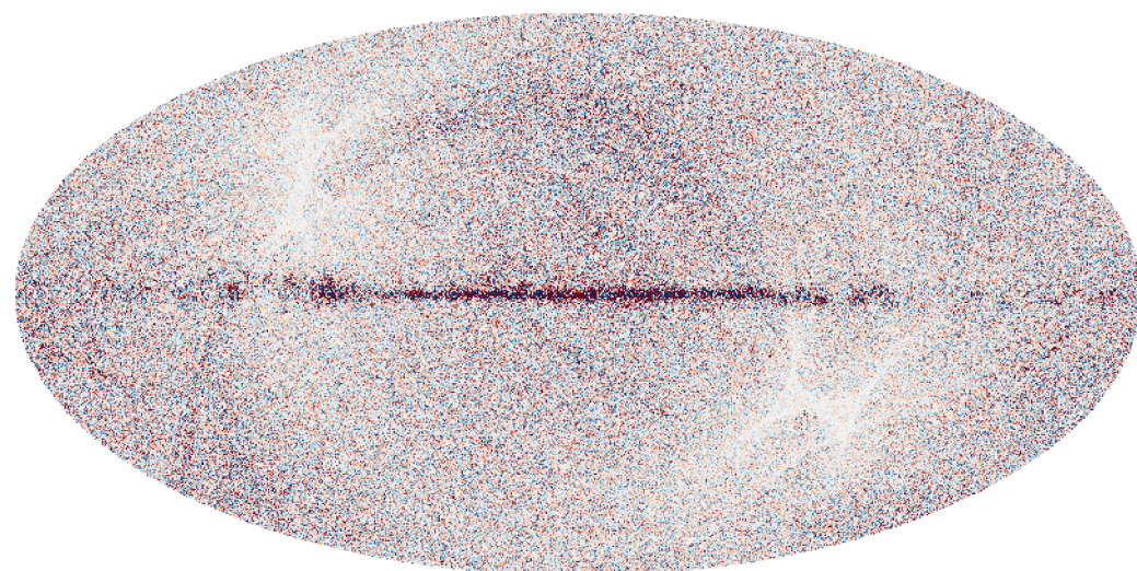
353 GHz NPIPE A mc_00200
