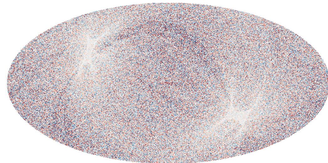
100 GHz NPIPE A mc_00200
