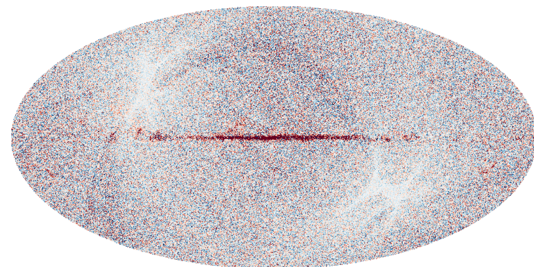
217 GHz NPIPE A mc_00200
