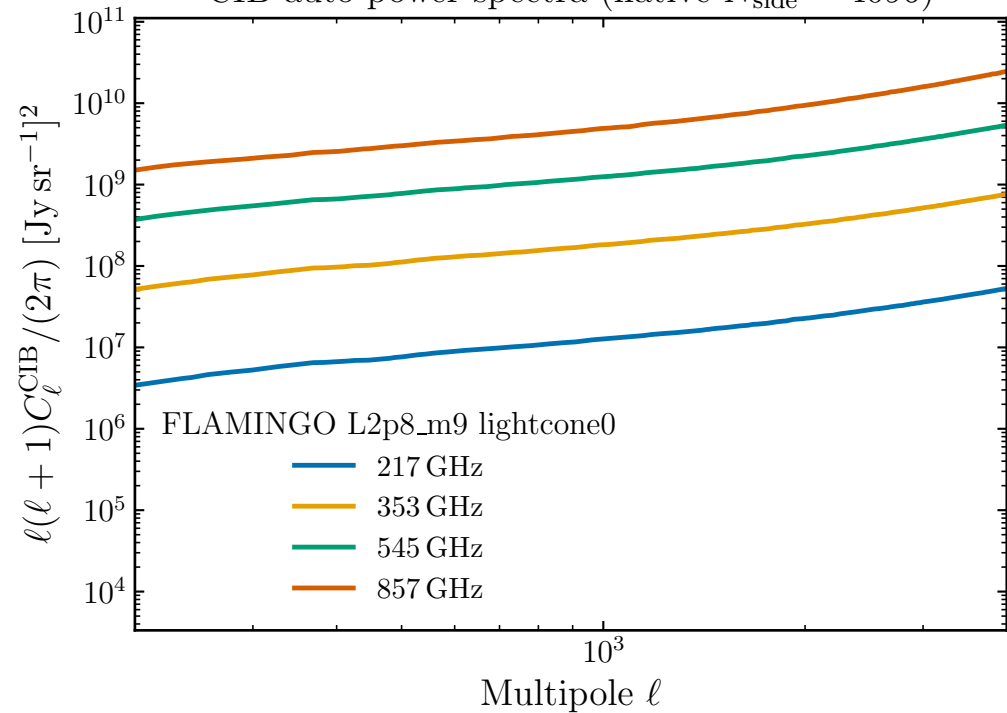
CIB auto-power spectra (native N_{\text{side}} = 4096 )
