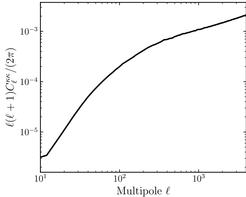
CMB lensing \kappa auto-spectrum
