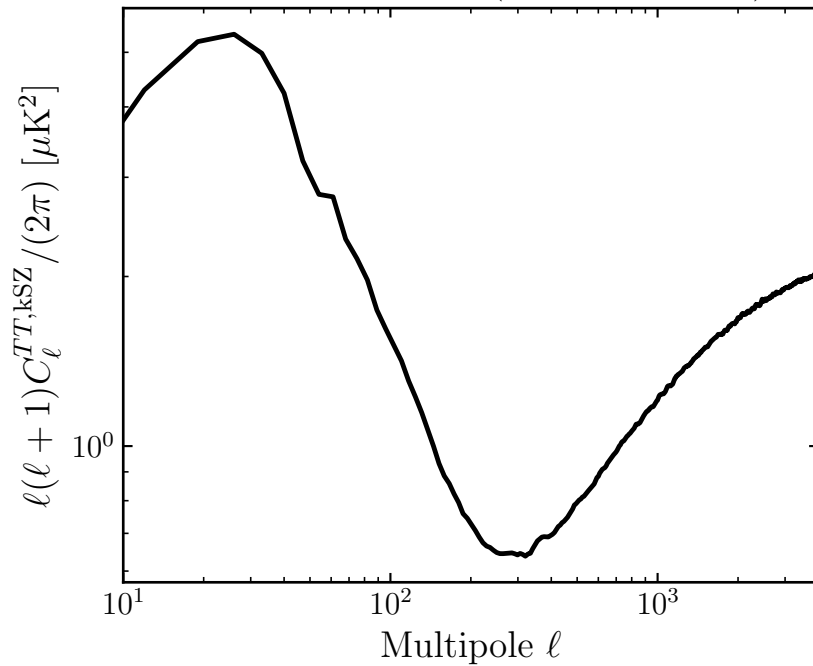
kSZ auto-spectrum (thermodynamic)
