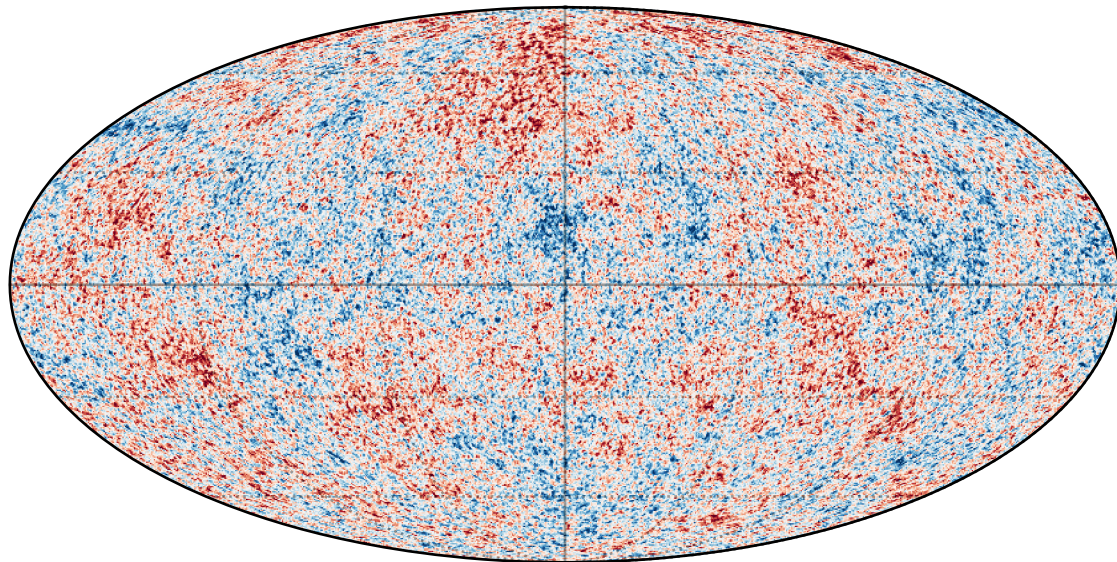
Lensed CMB
