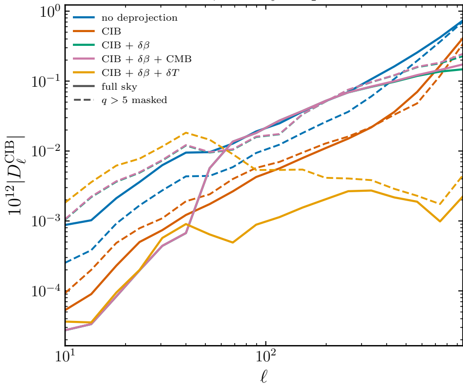
CIB residual, full sky vs q > 5 masked
