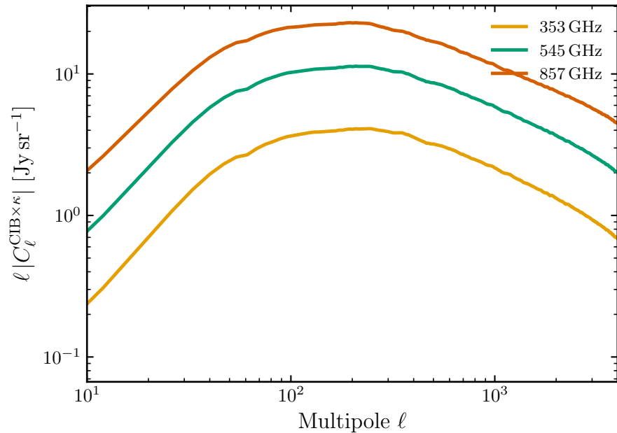
CIB- \kappa (cf. Fig. 10, right)
