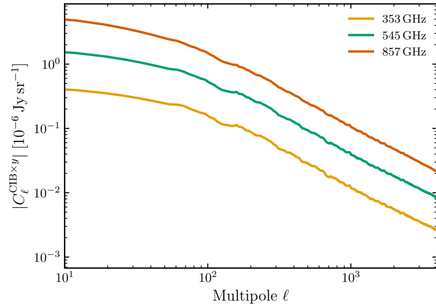
CIB-tSZ (cf. Fig. 10, left)
