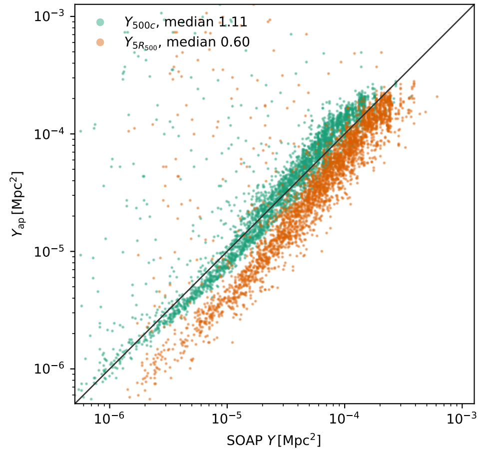
sky-avg W(\theta; \theta_{500}) , q > 5 , N = 3,090
