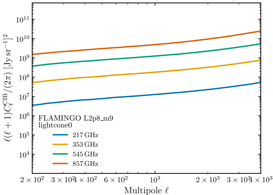
CIB auto-power spectra (native N_{\text{side}} = 4096 )
