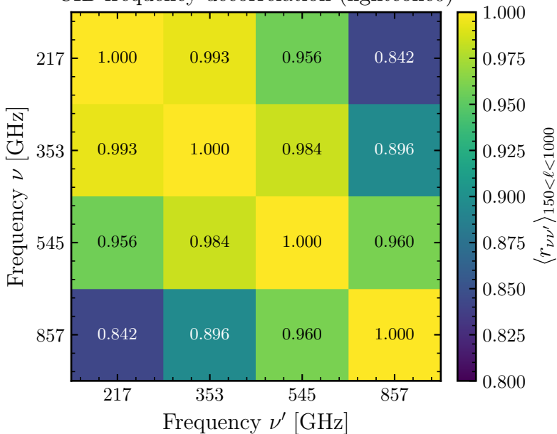
CIB frequency decorrelation (lightcone0)
