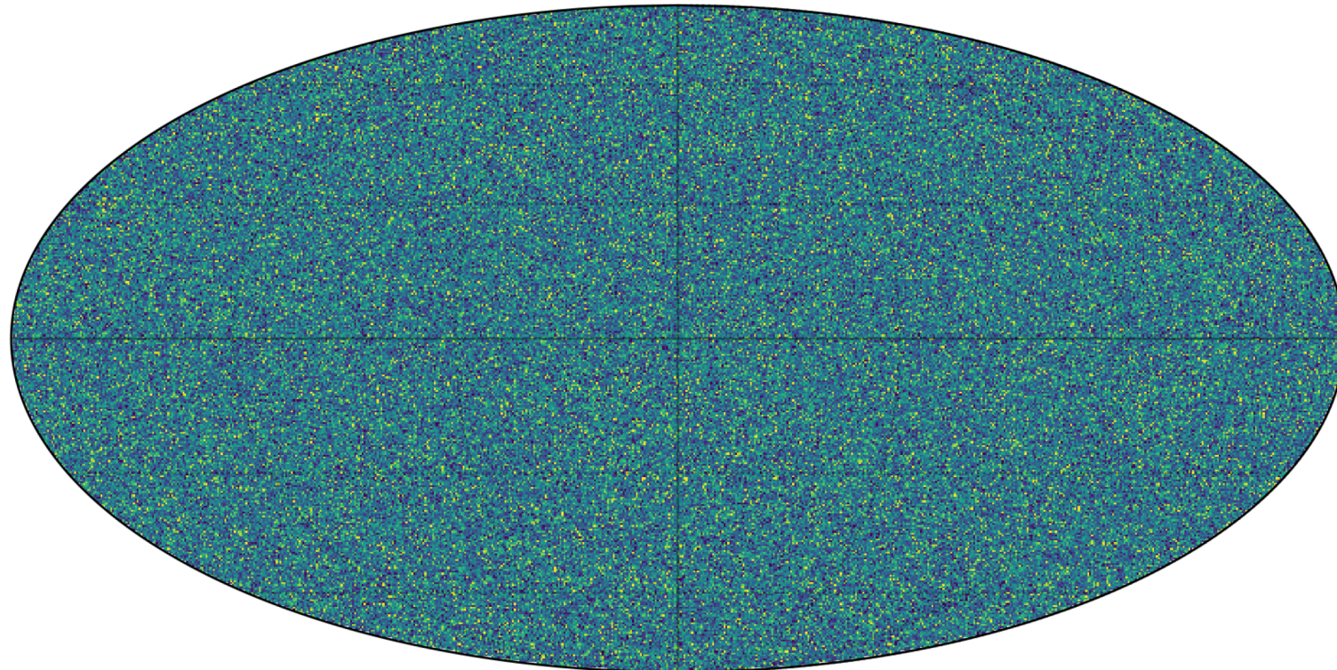
CIB \Delta T — 143 GHz (SED approx.)
