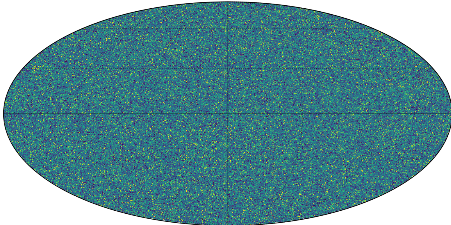
CIB \Delta T — 100 GHz (SED approx.)
