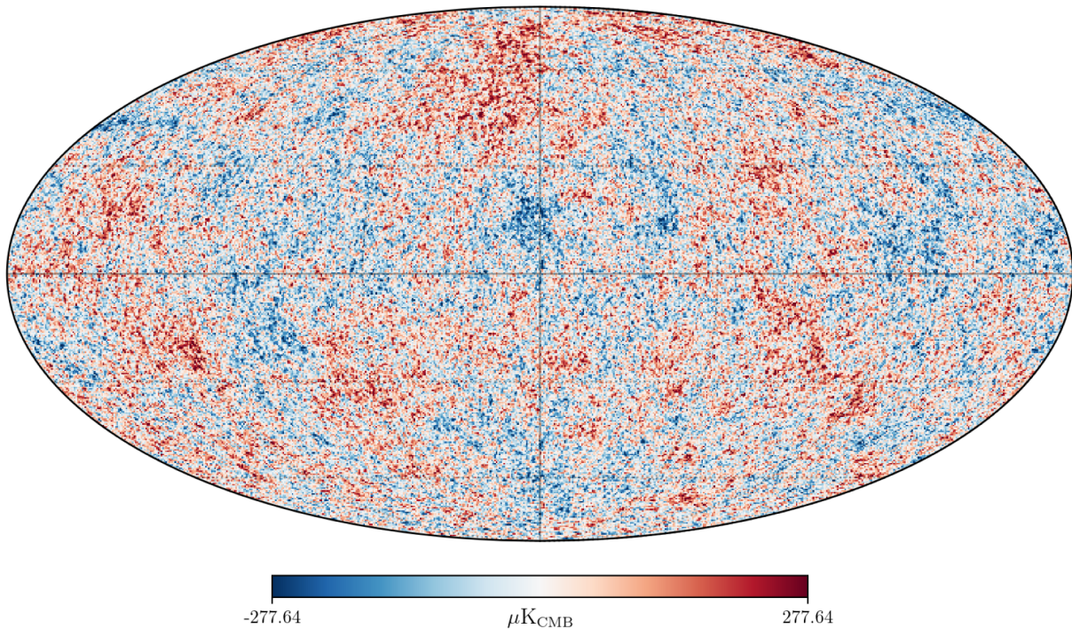
Lensed primary CMB ( N_{\text{side}} = 4096 )
