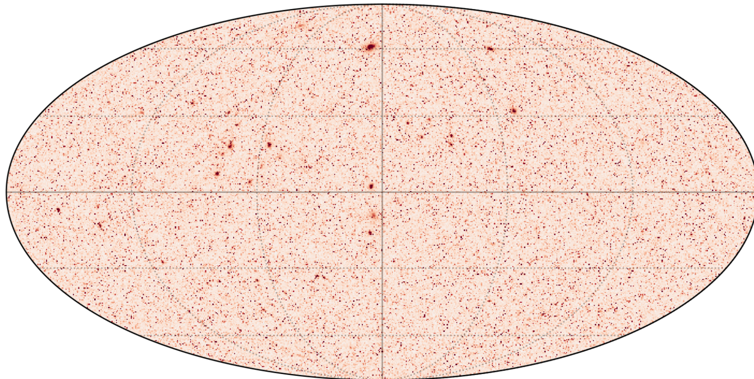
tSZ \Delta T at 545 GHz
