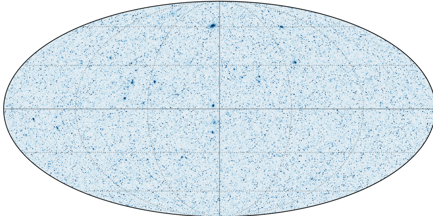
tSZ \Delta T at 143 GHz
