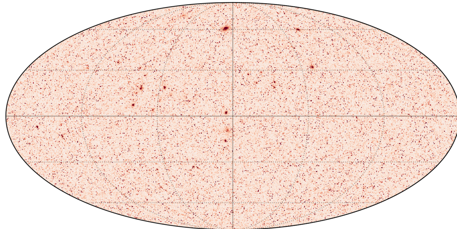
tSZ \Delta T at 857 GHz
