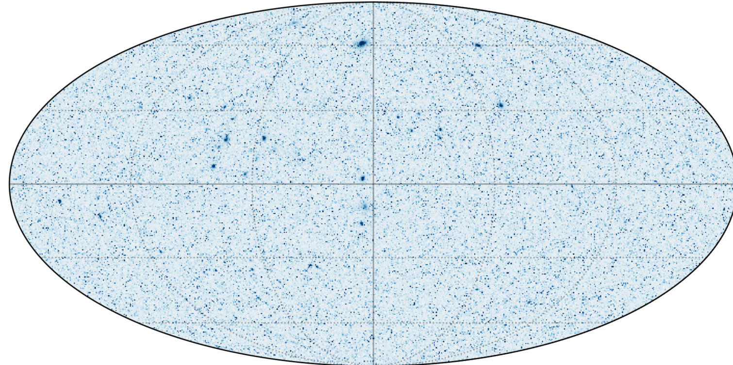
tSZ \Delta T at 217 GHz
