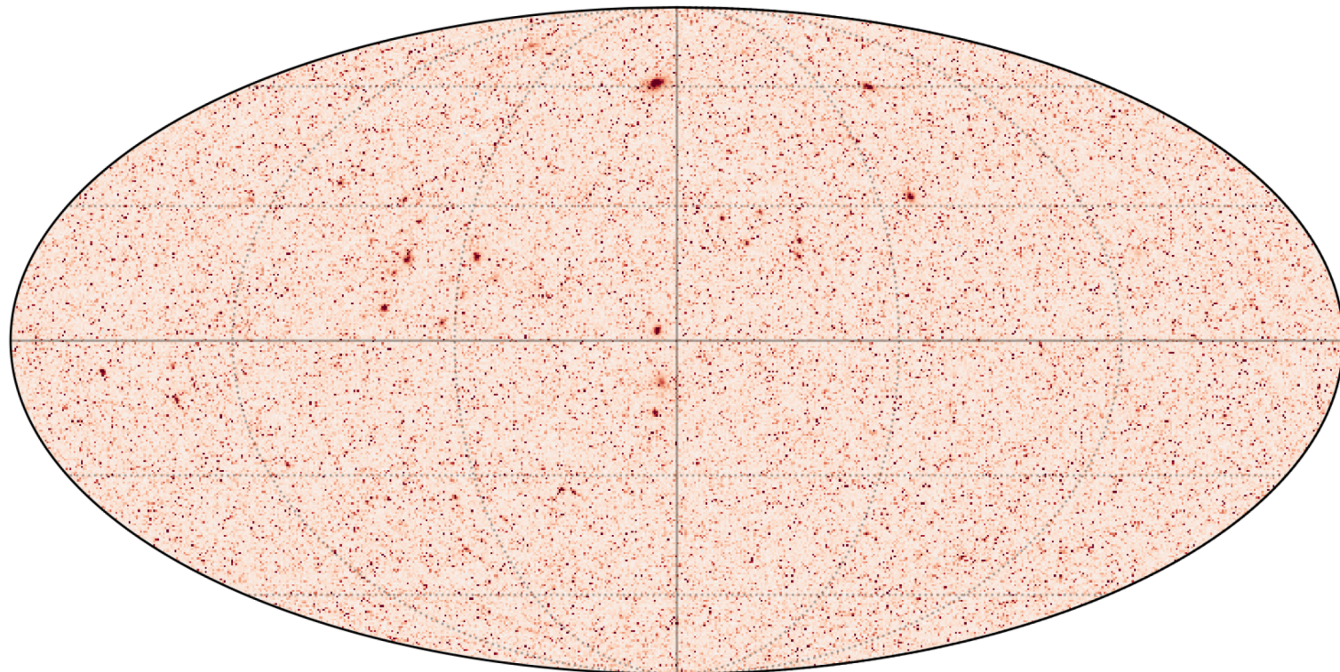
tSZ \Delta T at 353 GHz
