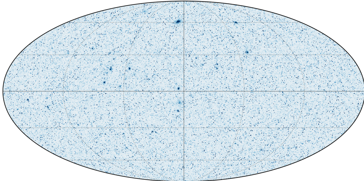
tSZ \Delta T at 100 GHz
