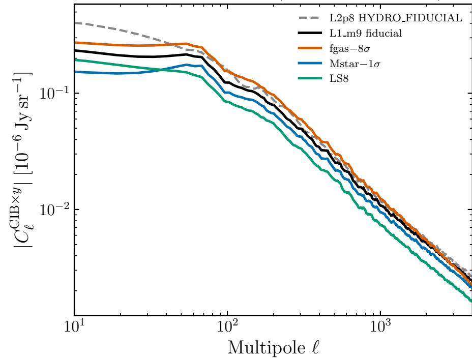
CIB-tSZ at 353 GHz (Yang26 Fig. 10 left)
