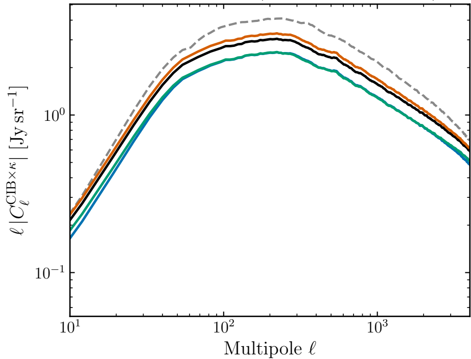
CIB- \kappa at 353 GHz (Yang26 Fig. 10 right)
