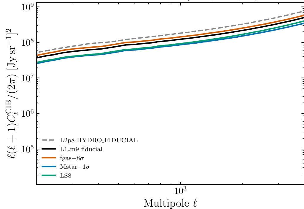
CIB auto at 353 GHz (Yang26 Fig. 8)
