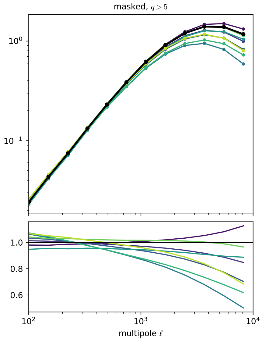
FLAMINGO L1_m9 feedback variants: tSZ power spectrum ( \Delta \ln \ell = 0.4 log bins; empirical aperture q )
