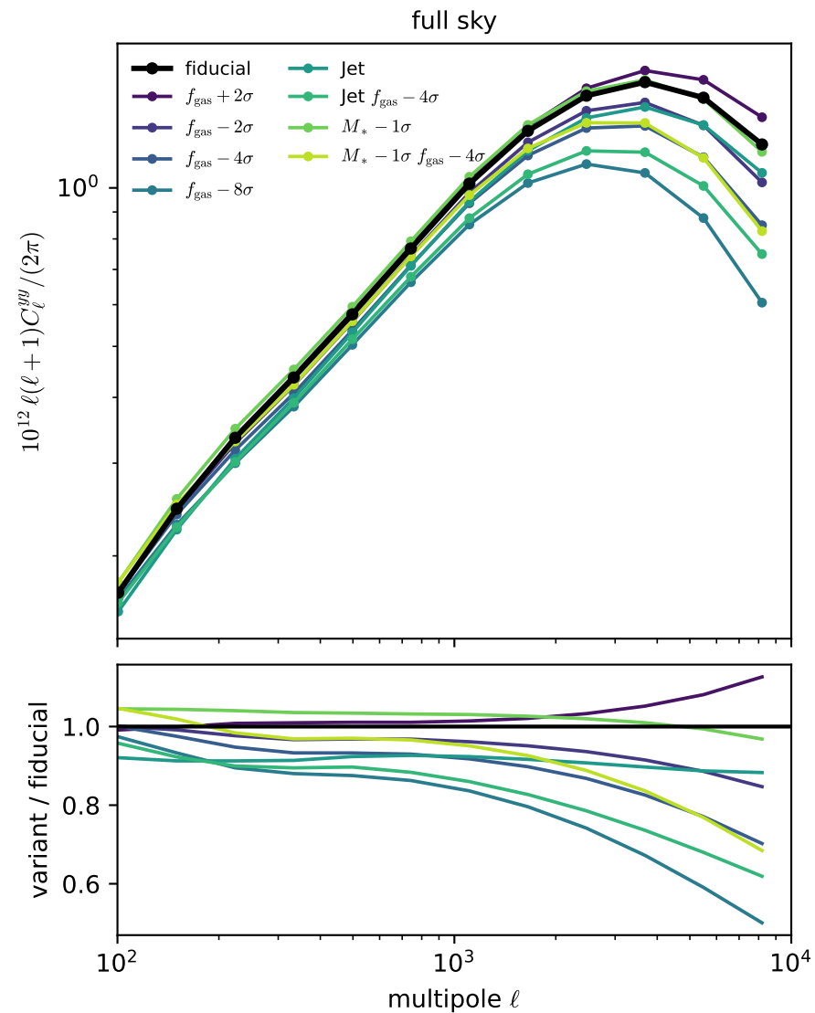
FLAMINGO L1_m9 feedback variants: tSZ power spectrum ( \Delta \ln \ell = 0.4 log bins; empirical aperture q )
