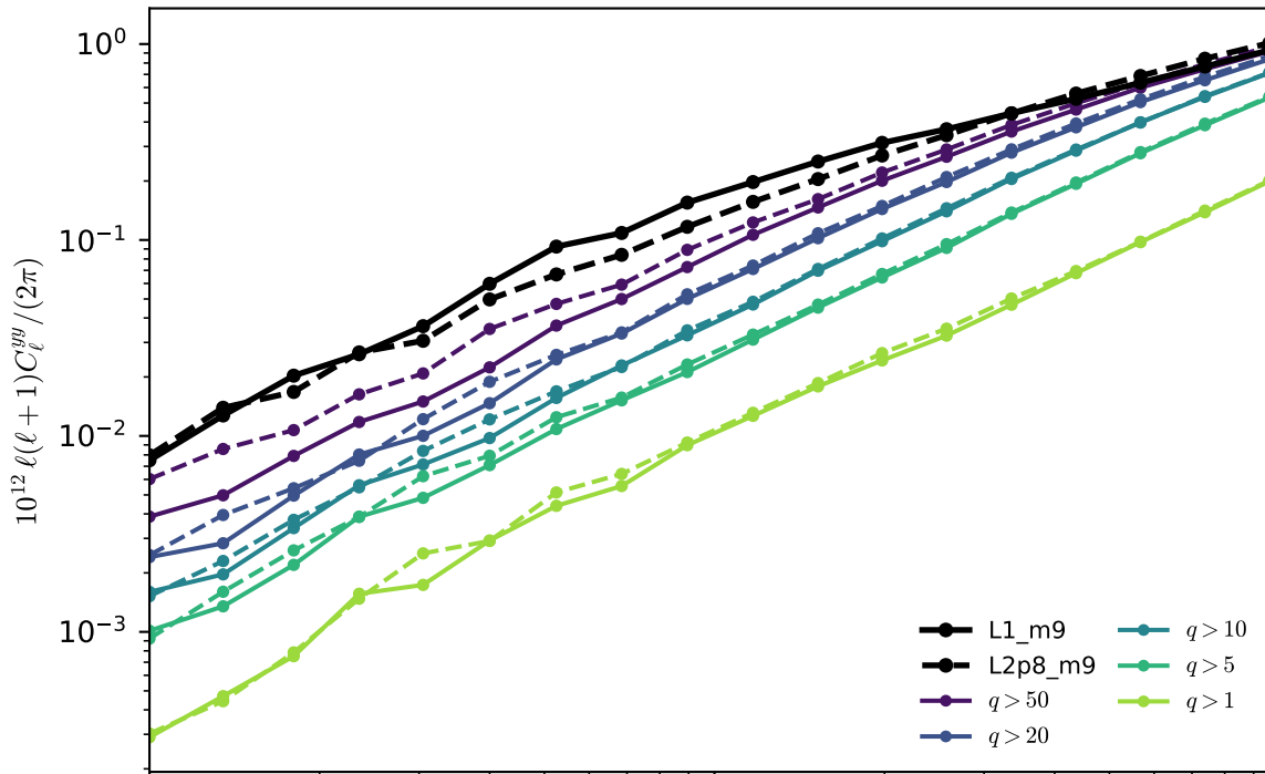
FLAMINGO masked tSZ: L1_m9 (solid) vs L2p8_m9 (dashed), 18 Planck bins, empirical aperture q
