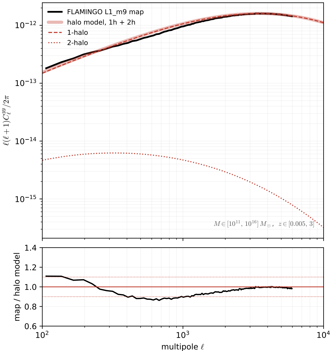
FLAMINGO L1_m9 total tSZ power spectrum vs. the A10 halo model ( B=1 , D3A)
