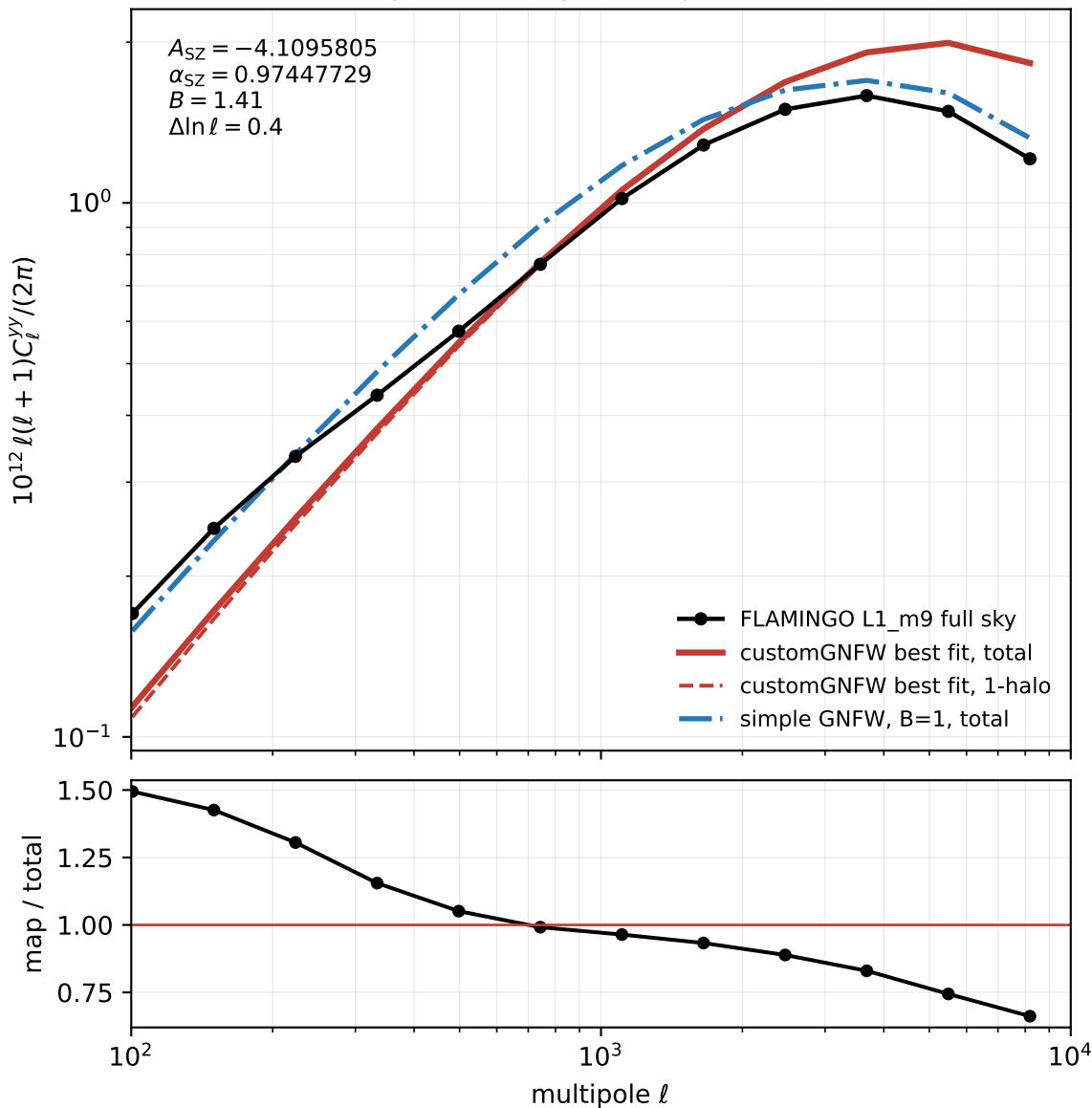
Full-sky total tSZ power spectrum (D3A)
