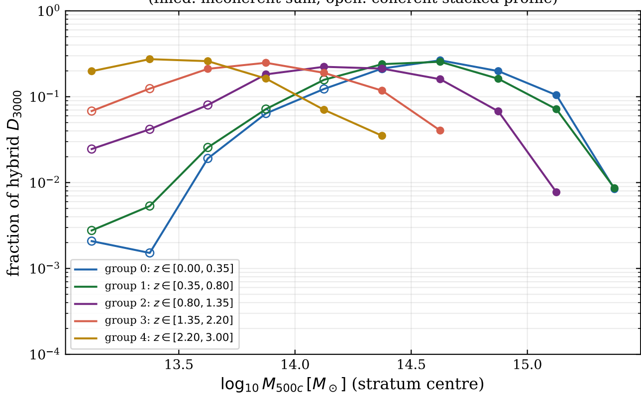
Mass-stratum contributions to the stacked D_{3000} (filled: incoherent sum; open: coherent stacked profile)
