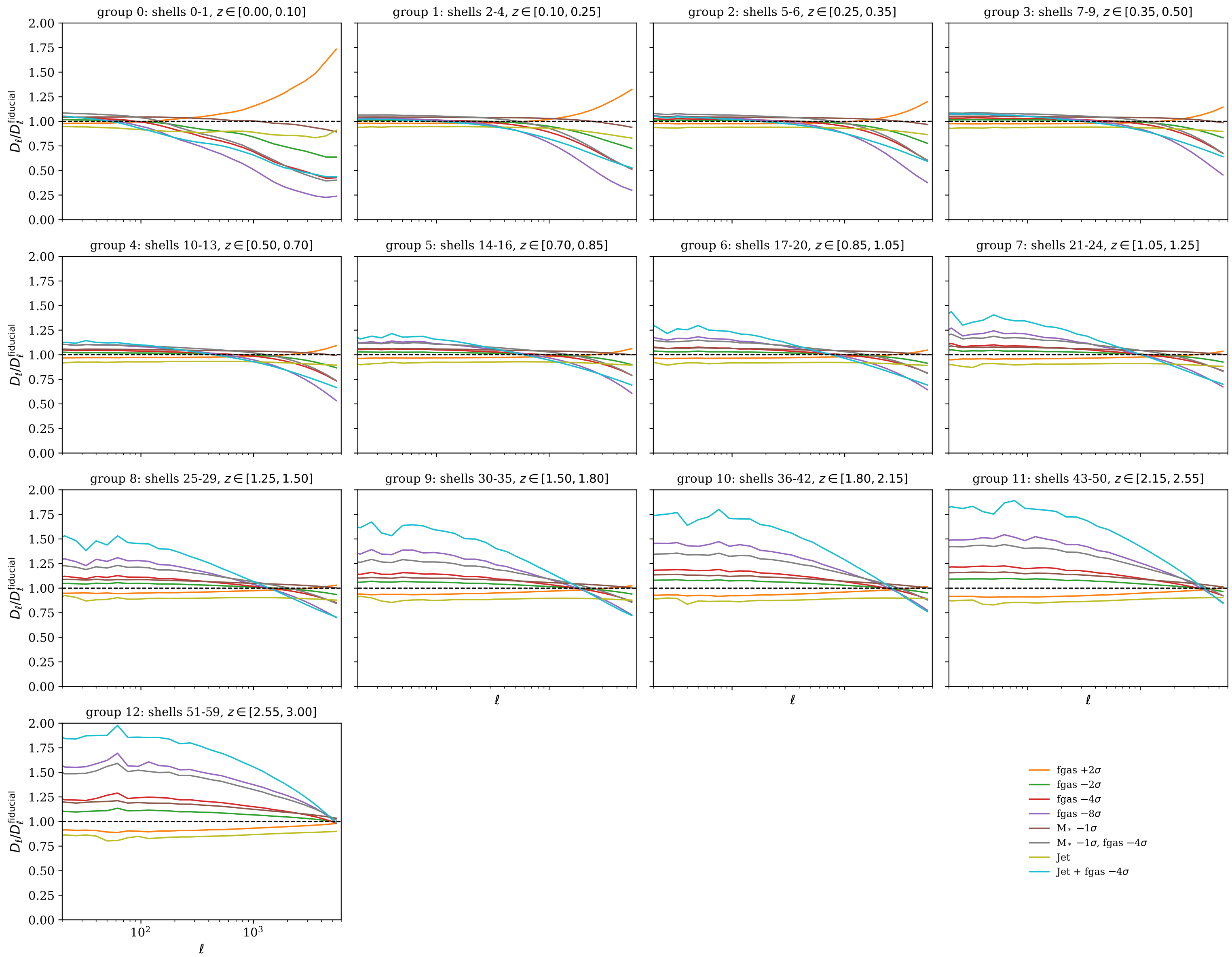
L1_m9 lc0 feedback variants: tSZ D_\ell ratio to fiducial per rotation group
