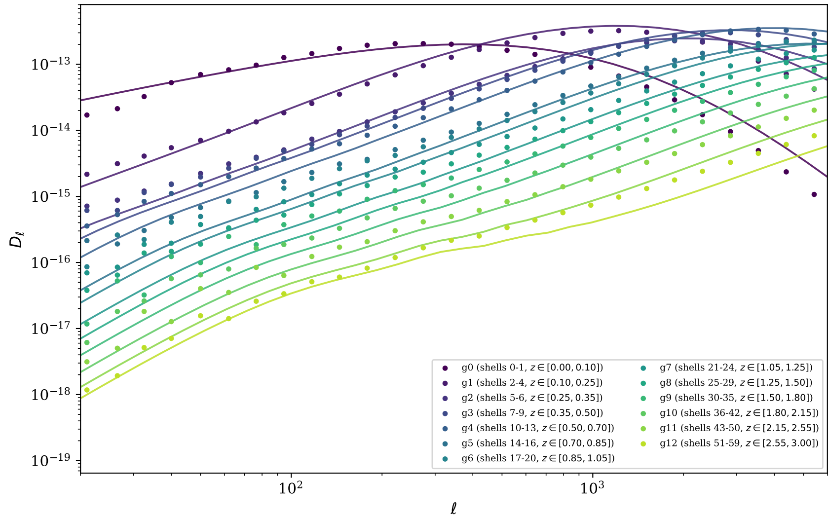
L1_m9 lc0 (fiducial): rotation-group tSZ D_\ell (points + theory lines)
