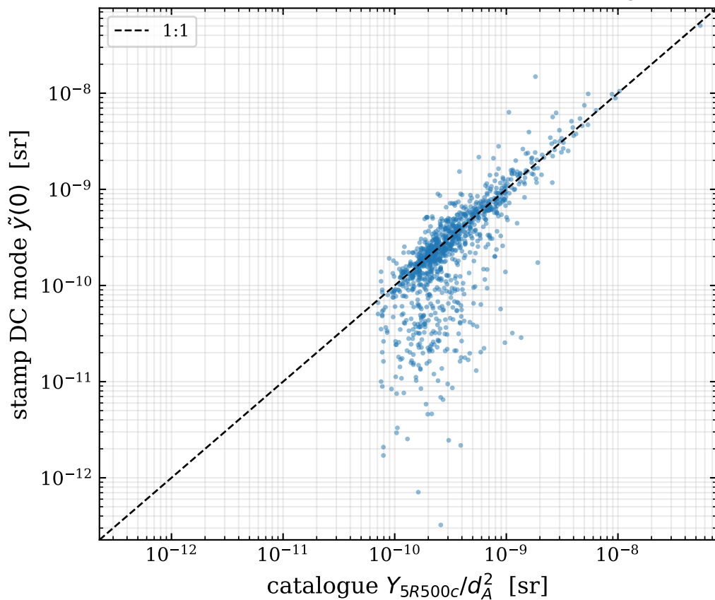
Per-cluster aperture \Upsilon : map stamps vs catalogue
