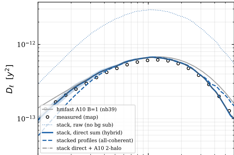
group 0: z \in [0.00, 0.35] , 4099 of 1,016,172 clusters
