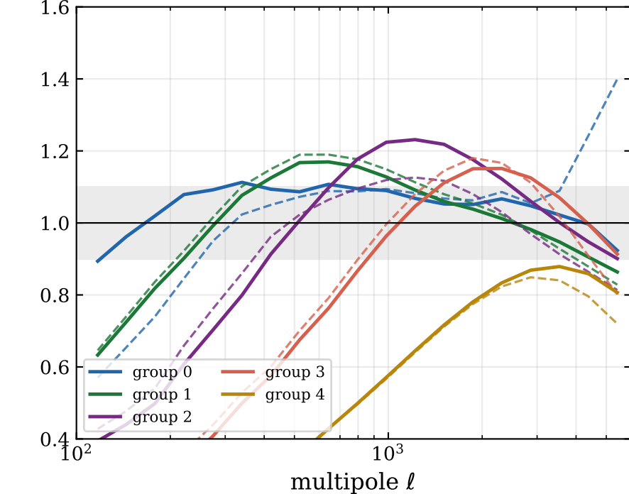
stack / measured (solid direct, dashed shape)
