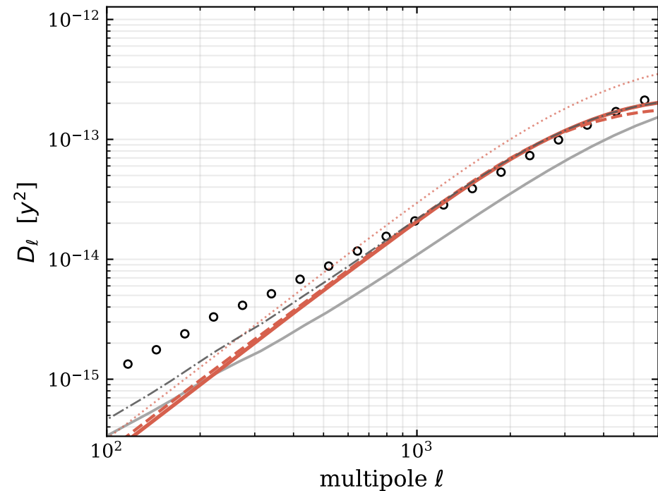
group 3: z \in [1.35, 2.20] , 3201 of 7,285,149 clusters
