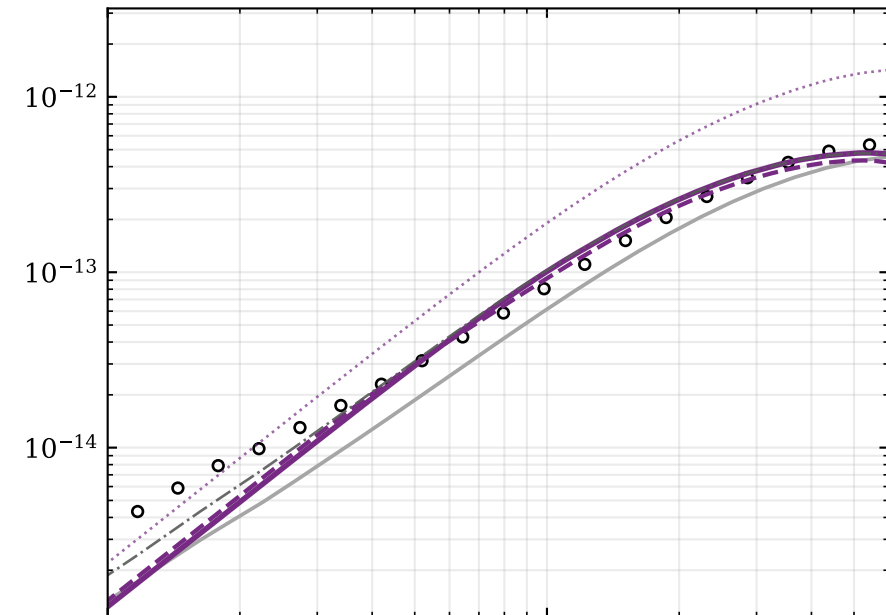
group 2: z \in [0.80, 1.35] , 3792 of 8,986,559 clusters
