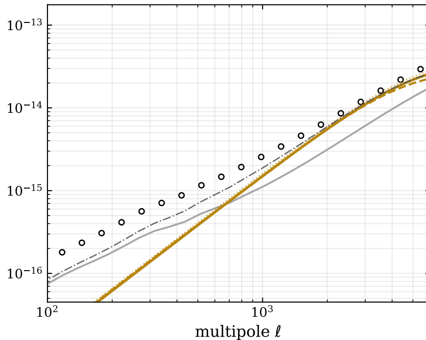
group 4: z \in [2.20, 3.00] , 2545 of 1,567,780 clusters
