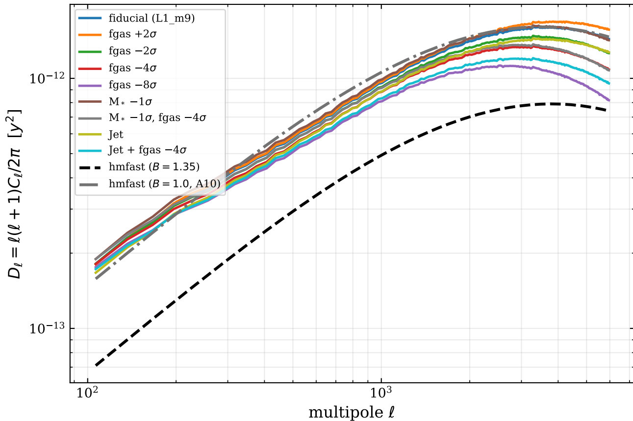
L1_m9 feedback: full sky (no q cut, no cluster mask)
