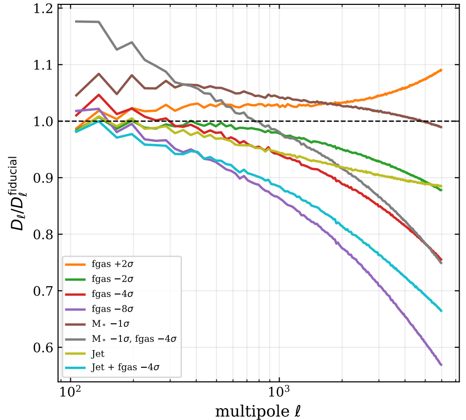
Masked q > 20 : ratio to fiducial L1_m9 ( q\_from\_mz > 20 )
