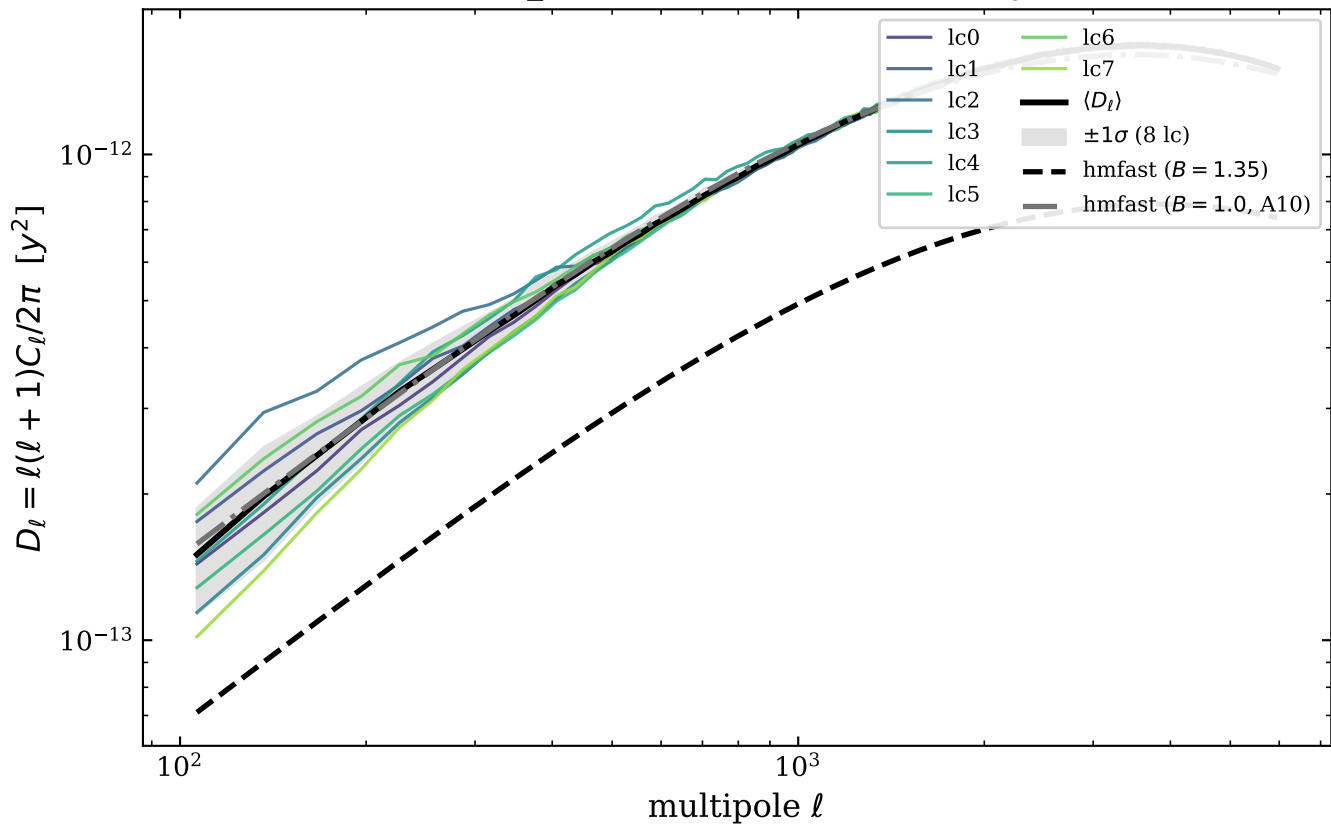
L2p8_m9 masked tSZ PS — Full sky
